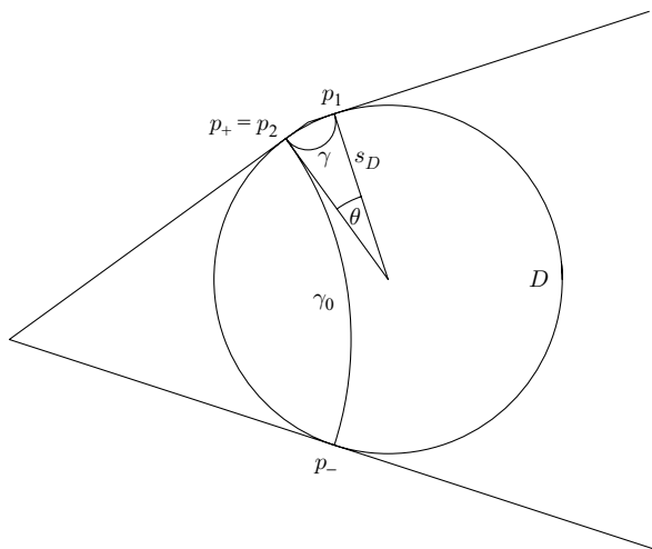
FIGURE 8.0. This picture illustrates the discussion in § 8. We have taken a case where, among all possible shapes of \Omega and among all possible configurations within \Omega , D happens to meet \partial_-\Omega : this makes s_D as large as possible consistent with our other assumptions. We have \gamma = r^{-1}(\lambda) and \gamma_0 = r^{-1}(\lambda_0) . The angle at the vertex on the left is approximately equal to \text{ang}(p) . We illustrate the special situation where p_2 and p_+ coincide. We also have D = D_0 and s_0 = s_D .
