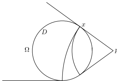
FIGURE 4.8. This illustrates (4.8.5). We show the convex set \Omega and a maximal disk D \subset \Omega . Two bending lines for \text{Dome}(\Omega) have a common endpoint x . The bending lines are not shown. Instead we show their inverse images under the nearest point retraction.
