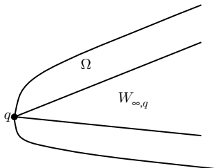
FIGURE 6.3. This illustrates Definition 6.3. We have q \in \partial\Omega . The region W_{\infty,q} \subset \Omega is the wedge defined in Definition 6.3.
