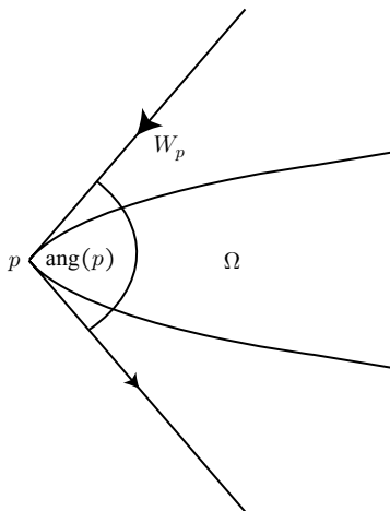
FIGURE 6.1. This illustrates Definition 6.1. The region W_p is the wedge contained between the two tangents to \partial\Omega at p . We have \Omega \subset W_p .
