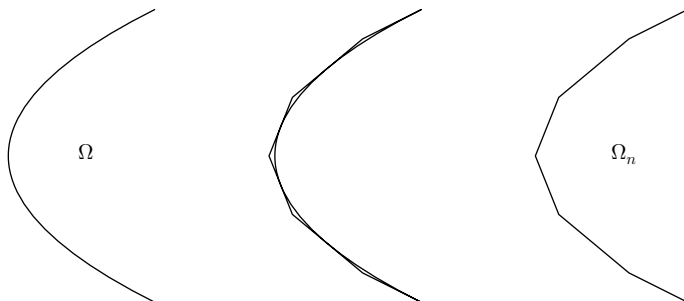
FIGURE 7.6. The left-hand figure is a convex curve, enclosing a convex region \Omega . The point p is at infinity on the right. The middle picture shows \Omega together with a number of support lines, as described in § 7.6. Using the support lines only, we obtain the polygonal approximation \Omega_n , as shown in the right-hand picture.
