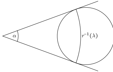
FIGURE 3.0.ii. This is a picture of the wedge whose dome is shown in Figure 3.0.i. The circle drawn is a circle that is maximal in the wedge. It is the boundary of the hyperbolic plane which contains the geodesic \lambda and is tangent to the cone surface. This hyperbolic plane is a hemisphere. The diagram has been rescaled so that the corresponding sphere has radius 1. We choose coordinates so that the wedge vertex is the origin. Then S = (\cot(\alpha/2), 0, -1) is the lowest point of that corresponding sphere. The nearest point retraction r : r^{-1}(\lambda) \rightarrow \lambda is given by radial projection from S .
