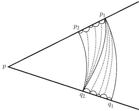
FIGURE 9.0. This illustrates §9, where the bending lamination is extended to a foliation of a neighbourhood of p by geodesics. The picture should really be drawn on \text{Dome}(\Omega) , but we have instead drawn the inverse image in \Omega under the nearest point retraction r , which is easier to do. Notice the small fringe geodesics. For convenience, we have drawn the boundary of \Omega in two straight pieces, but we must have some deviation from straightness if there is to be any fringe. The solid curves are inverse images of bending lines. The dotted curves are inverse images of the new geodesics introduced in order to create a foliation.
