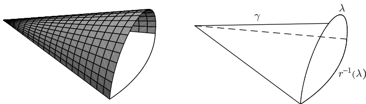
FIGURE 3.0.i. The dome of a wedge is a cone. In the left-hand picture, the mesh shown consists, on the one hand, of semicircles orthogonal to the plane \{z = 0\} and, on the other hand, rays through the origin. The semicircles are hyperbolic geodesics in \mathbb{H}^3 . The rays are not geodesics in \mathbb{H}^3 . However, the ray \gamma , running along the highest points of the semicircles, is a geodesic for the induced Riemannian metric on the dome. One of the semicircles is labelled \lambda , in agreement with the surrounding text, and its inverse image r^{-1}(\lambda) under the nearest point retraction r is also labelled.
