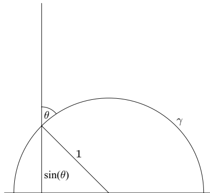
FIGURE 9.1. This diagram illustrates the proof of Lemma 9.1. We show the geodesic \gamma of that proof as a semicircle of radius 1 in the upper half-plane. We work out the relationship between the signed distance t measured along \gamma , and the angle that a vertical geodesic makes with \gamma . Since the point of interest is at height \sin(\theta) , we see that dt = d\theta / \sin(\theta) .
