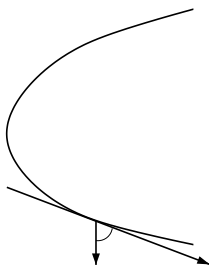
FIGURE 7.3. This illustrates the first paragraph of §7.3.
