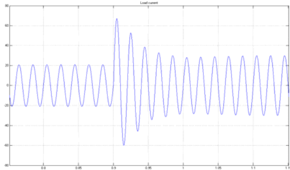
Fig. 9: Line-sensitive-equipment current
