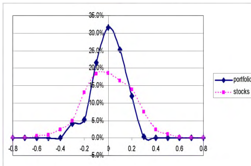
Figure 1 Beta Change Distribution
