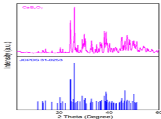
Figure 1 XRD patterns of \text{CaB}_4\text{O}_7 compound
