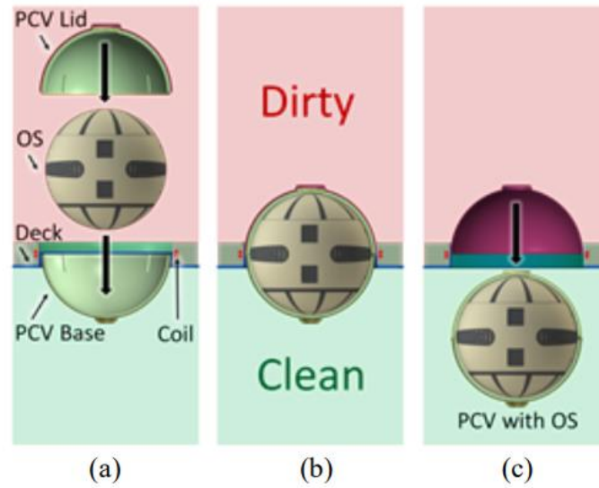
Figure 2. Illustration of an inductive brazing sequence. (a) OS assembled with the PCV Lid to the PCV Base brazed to the Deck. (b) Inductive brazing operation simultaneously brazes together the PCV Lid outer wall to the Deck, brazes together the PCV Lid inner wall to the PCV Base, separates the PCV Lid inner wall from the PCV outer wall, separates the PCV Base from the Deck, and sterilizes all regions along and in between the brazing surfaces. (c) PCV Lid inner wall, the OS, and the PCV Base removed from the Deck (Younse et al. , 2018).
