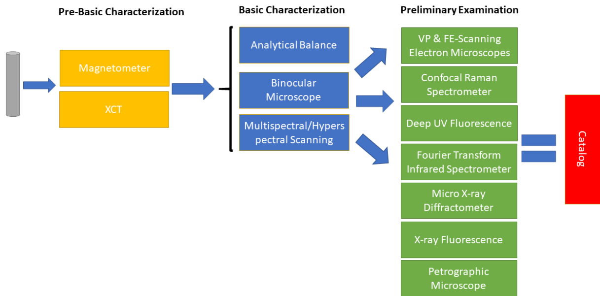
Figure 5. Proposed list of instrumentation for Pre-Basic Characterization, Basic Characterization, and Preliminary Examination to produce a sample catalog.
