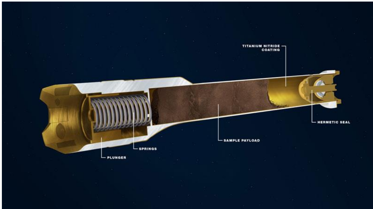
Figure 1. This illustration depicts the interior of a sample tube being carried aboard the Mars 2020 Perseverance rover. About the size and shape of a standard lab test tube, the 43 sample tubes headed to Mars are lightweight, hardy enough to survive the demands of the round trip, and so clean that future scientists will be confident that what they are analyzing is 100% Mars, without terrestrial contaminants. Credit: NASA/JPL-Caltech.
