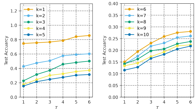
Figure 4: Analysis of TP-MANN’s number of recurrent-layers ( T ). The x-axis is T with which the model has been trained. Each line represents a different value of k of the StepGame dataset.
