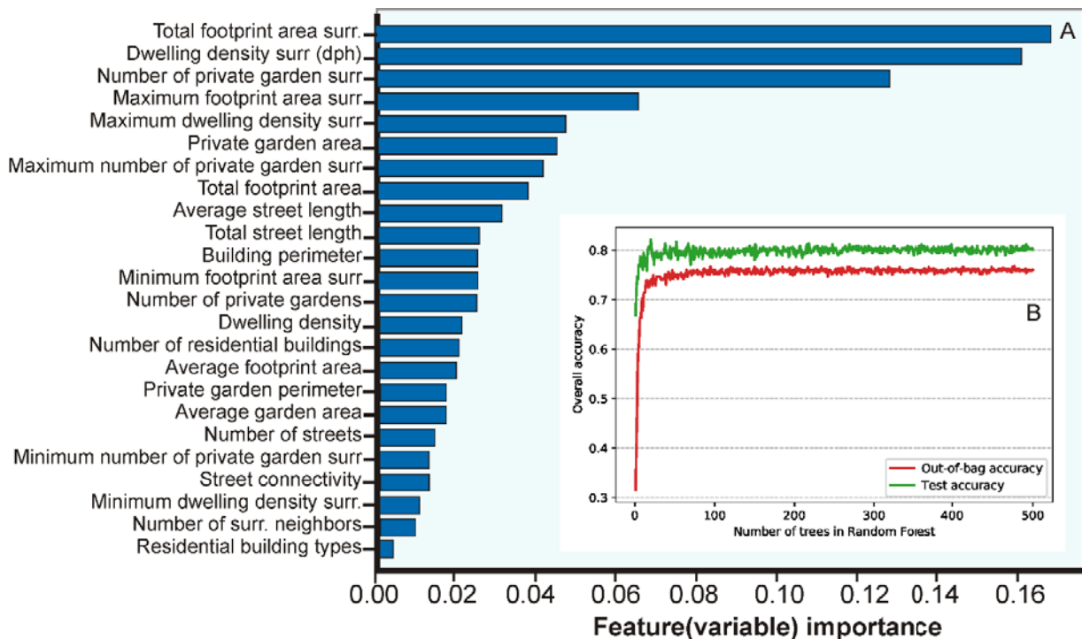
Figure 2. (A) Variable (feature) importance. The graph shows the importance of each variable during the RF training for the classification of urban forms. Surr. in the figure refers to the surroundings. (B) the graph show the Out-of-bag accuracy and test accuracy for 500 trees in Random Forest.
