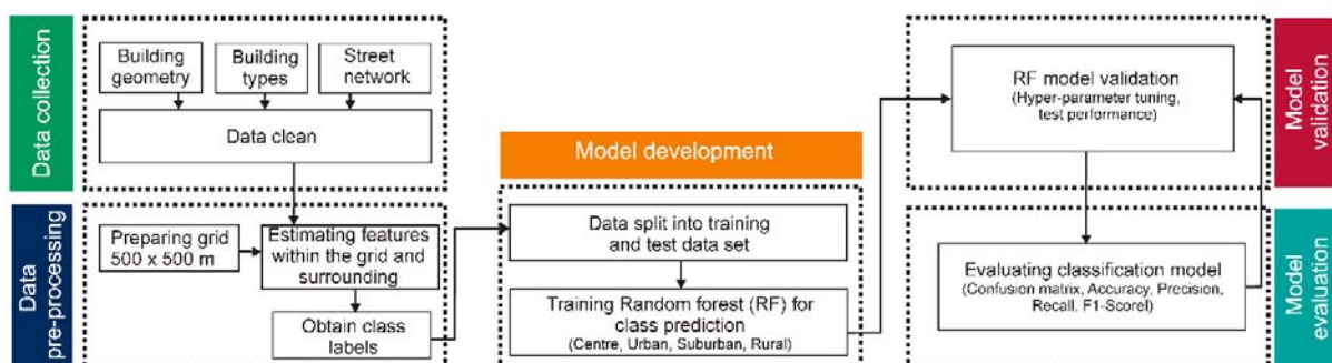
Figure 1. Workflow for classification modelling of residential neighbourhoods
