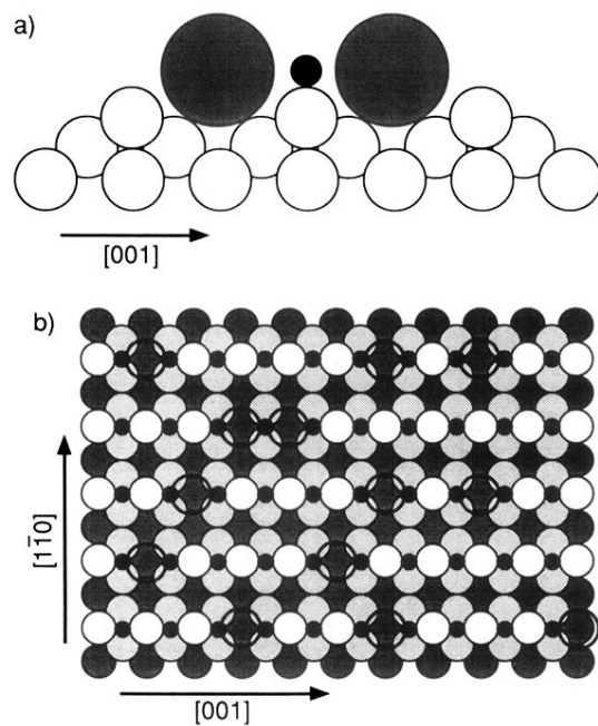
FIG. 4. (a) Schematic model of a \text{K}_2\text{O} unit in the (1 \times 2) missing-row reconstruction; (b) model of the (2 \times 1)\text{O}/\text{alkali}/\text{Cu}(110) reconstruction (small black circles: oxygen atoms; medium sized circles: Cu atoms; larger, transparent circles: alkali-metal atoms).
