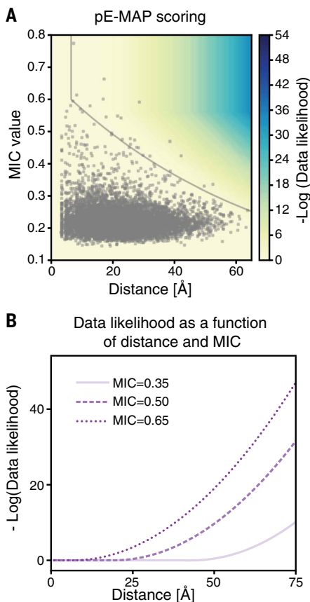
Fig. 4. Generation of the scoring function.
