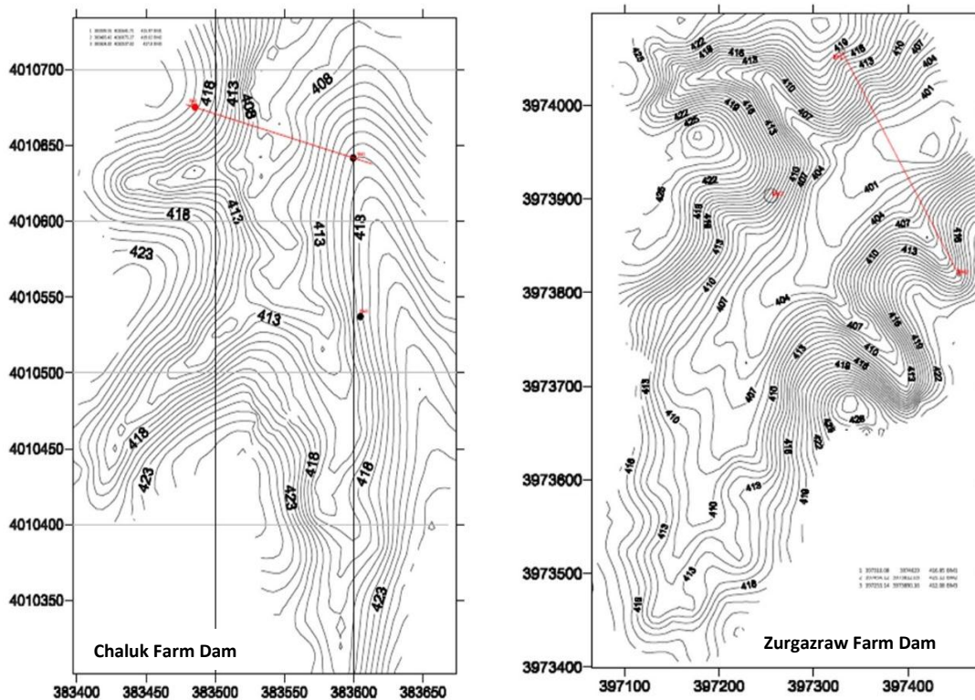
Figure 1: Contour Maps of Proposed Farm Dams
