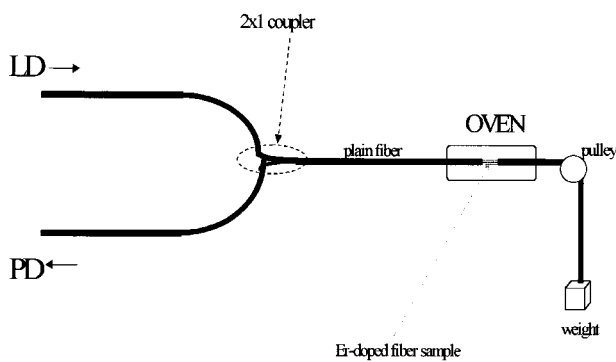
FIG. 1. Experimental arrangement used in this work.
