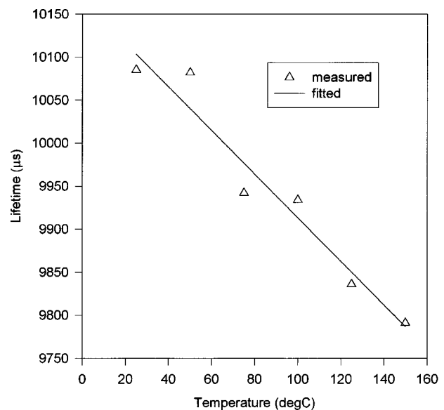
FIG. 3. Graph of fluorescence lifetime vs temperature.
