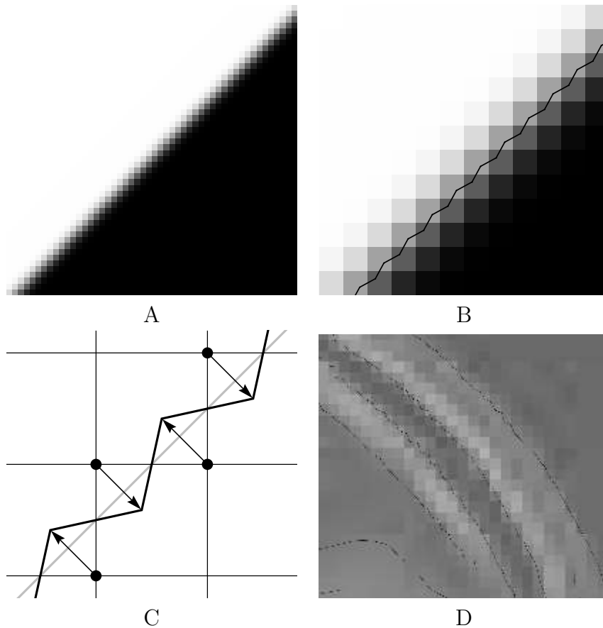
Figure 9: A Synthesized Gaussian edge at 45 degrees, with \sigma = 1 , and an offset of \gamma = \frac{\sqrt{2}}{4} . B A detail of the synthesized edge in A and the detected edges by the Devernavy method. An oscillatory pattern is observed. C An scheme explaining the reason of the oscillatory pattern. The true edge is located exactly at mid distance between the two sets of diagonal grid points. By symmetry, all the points marked by dots are local maxima. The arrows show the offsets \eta computed by the Devernavy method. The errors appear in alternate directions, creating the observed oscillations. D Detail of the upper-right side of Figure 10 of the original work by Devernavy [5], showing that the “oscillatory” patterns were indeed present in the original implementation of the method.
