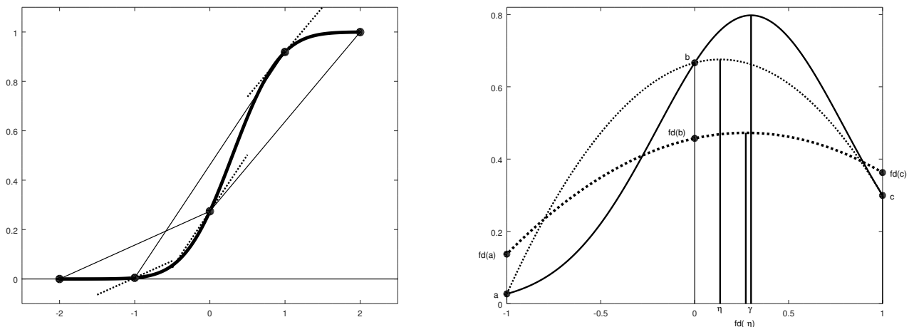
Figure 6: Partial compensation of errors in a Gaussian edge for \sigma = 0.5 and \gamma = 0.3 . Left: The Gaussian edge profile (thick line) and the finite difference estimations of the derivatives (dotted lines) by centered difference (thin lines). The finite difference estimations of the derivative are larger than the actual ones at positions -1 and 1 ; the estimation gives a smaller value at 0 . Right: The exact gradient profile (solid line) with its maximum at \gamma ; the parabolic approximation using the exact derivative values a , b and c (thin dotted lines) with its maximum at \eta ; the parabolic approximation using the derivatives fd(a) , fd(b) and fd(c) estimated by finite differences (thick dotted line) with its maximum at fd(\eta) . Note that the errors due to the finite difference estimation of the gradient compensate in part the error of the parabolic approximation, reducing the final error.
