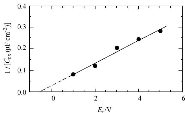
Figure 3. Inverse of the oxide capacitance C_{ox} as a function of the formation potential E_f (vs. sce ), for thin anodic Nb 2 O 5 films formed on Nb electrodes in 0.5 mol/L H 3 PO 4 (pH 1.3).
