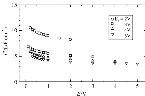
Figure 4. Capacitance of metal/passive film/electrolyte system as a function of the applied potential E (vs. sce ), for thin anodic Nb 2 O 5 films formed on Nb electrodes at different formation potentials E_f in 0.5 mol/L H 3 PO 4 (pH 1.3).
