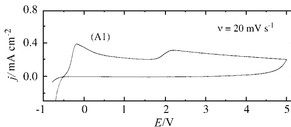
Figure 1. Voltammogram of Nb in 0.5 mol/L H 3 PO 4 (pH 1.3) obtained between E_{s,c} = -0.8 V and E_{s,a} = 5 V ( vs. sce ) at v = 20 mV s -1 .
