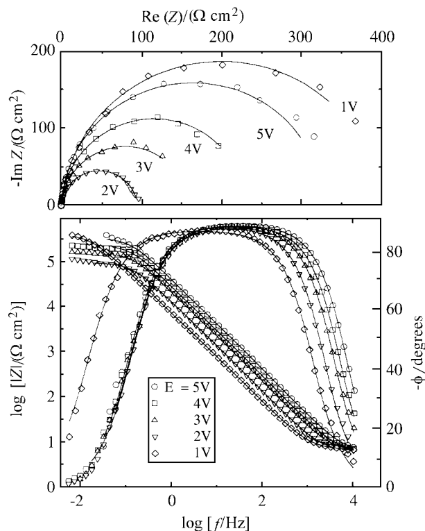
Figure 2. Complex-plane and Bode plots obtained for thin anodic \text{Nb}_2\text{O}_5 films formed on Nb electrodes at different formation potentials E_f (vs. sce ) in 0.5 mol/L \text{H}_3\text{PO}_4 (pH 1.3). The lines correspond to calculated impedance data according to a transfer function (see text).
