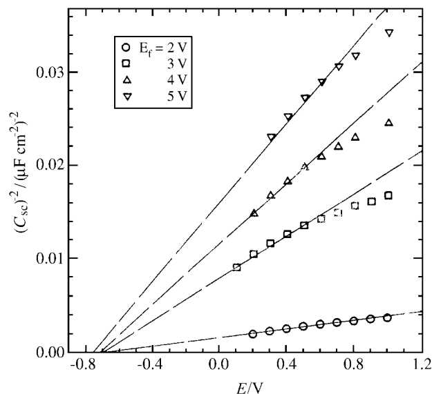
Figure 5. Mott-Schottky plots for thin anodic Nb 2 O 5 films formed on Nb electrodes in 0.5 mol/L H 3 PO 4 (pH 1.3), at the indicated formation potentials E_f (vs. sce).
