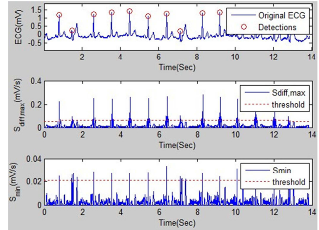
Fig. 5. QRS detection over tape 202 of the MIT/BIH database with sharp changing peak amplitudes.
