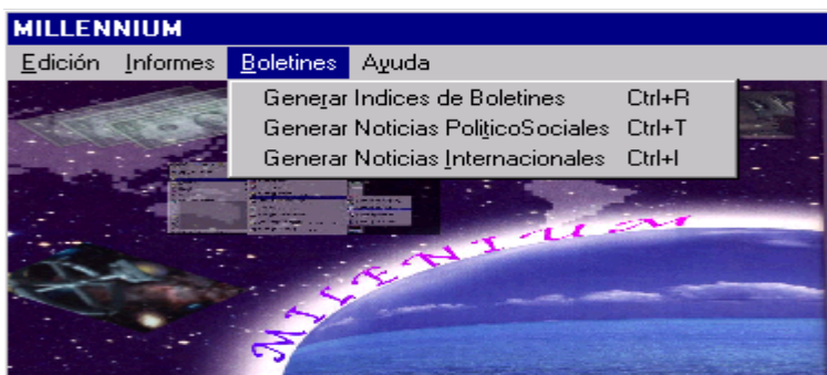
Figura 6.19 Menu Boletines
