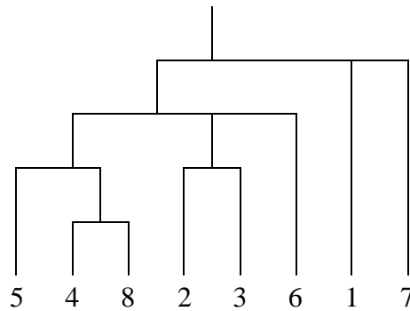
Figure 2. Dendrogram formed by the between farms similarity matrix.
