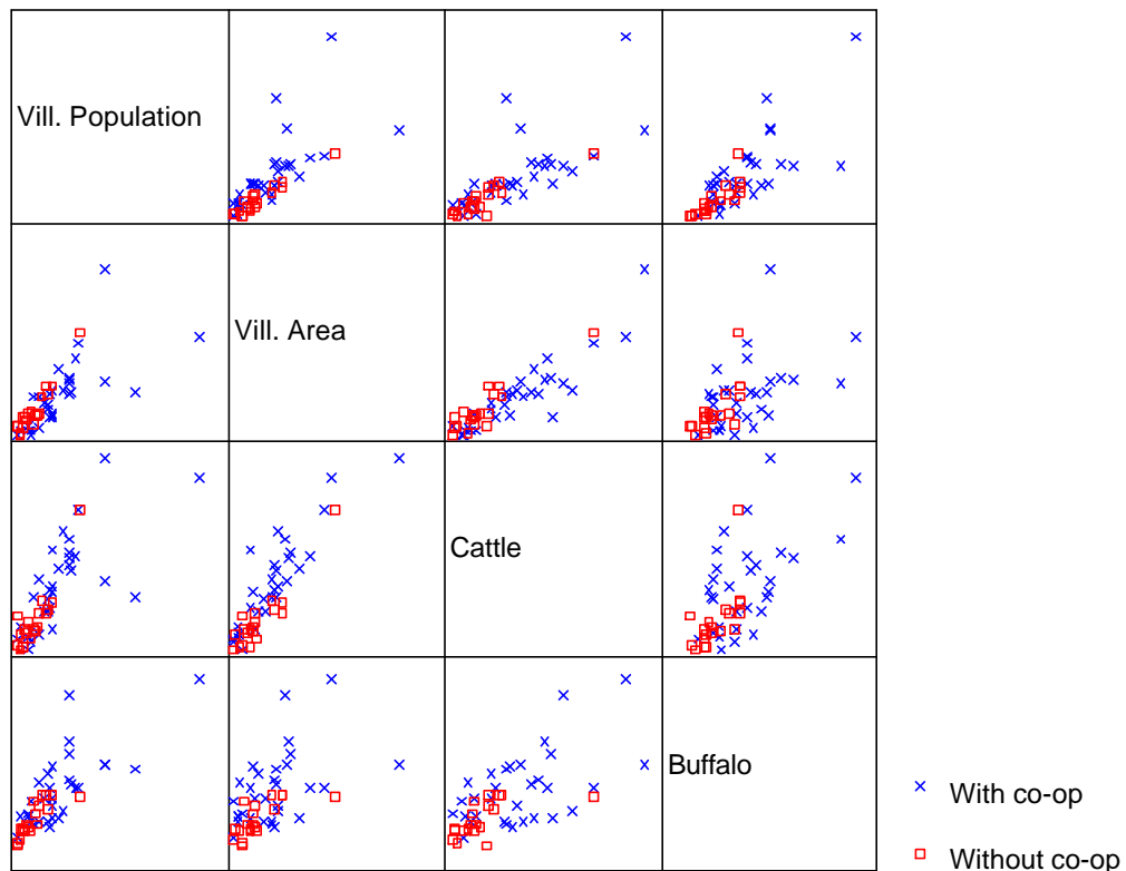
Figure 1. An example of a matrix plot amongst six variables.
