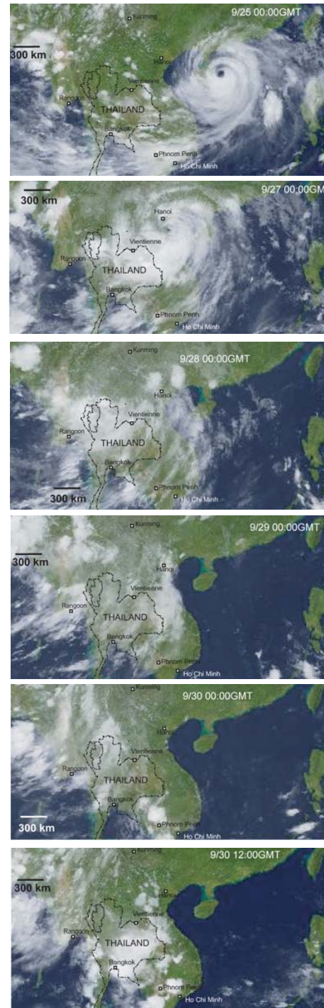
Fig. 3. Satellite images showing the westward traveling tropical storm from Typhoon Damrey, 25–30 September 2005. From archive of EEI-lab, Kochi University, MTSAT IR1 JMA. Thailand local time is 7 h later than GMT.
