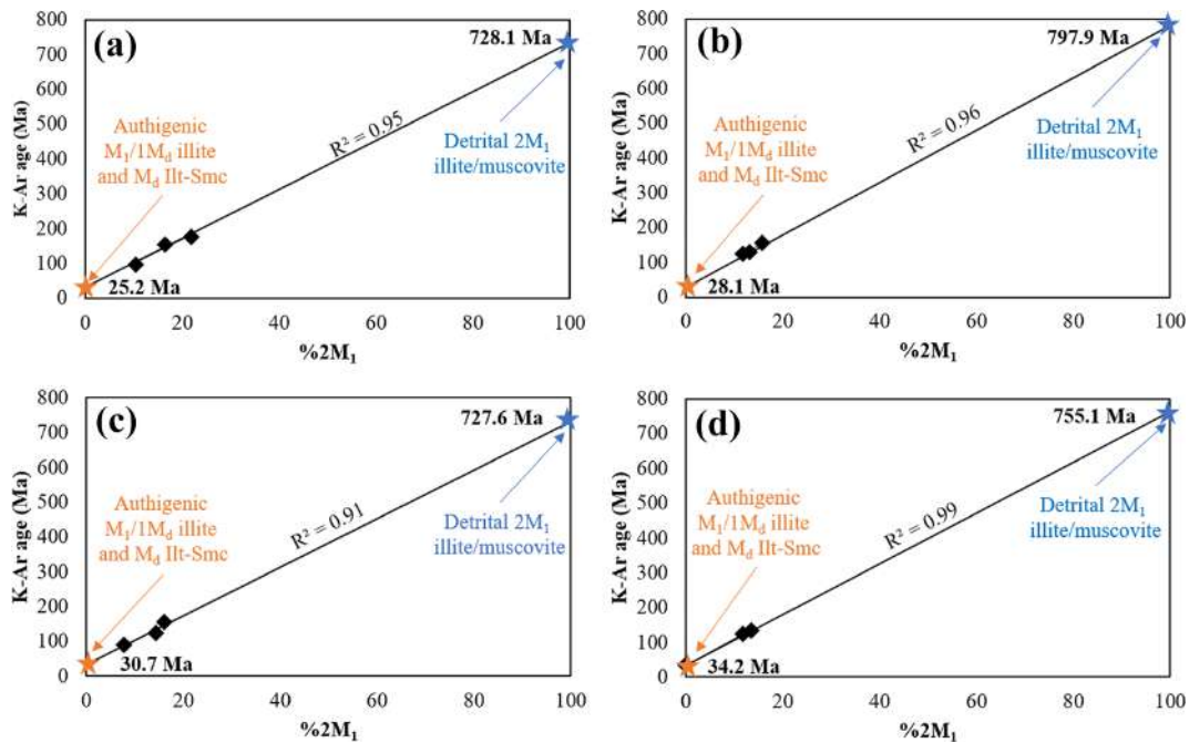
Figure 5. Crystallization ages of detrital 2M_1 illite/muscovite and of authigenic 1M_d/1M illite and illite–smectite (Ill–Smc) from the Valley of Lakes, calculated for sediments collected from the (a) TAT section ( \sim 90.5 m), (b) TGR-C section ( \sim 78.0 m), (c) SHG-D section ( \sim 55.5 m) and (d) TGR-AB section ( \sim 35.0 m) using illite polytype quantification and K–Ar age systematics of different grain size subfractions (from left to right: <1 , 1\text{--}2 and 2\text{--}10\ \mu\text{m} ).
