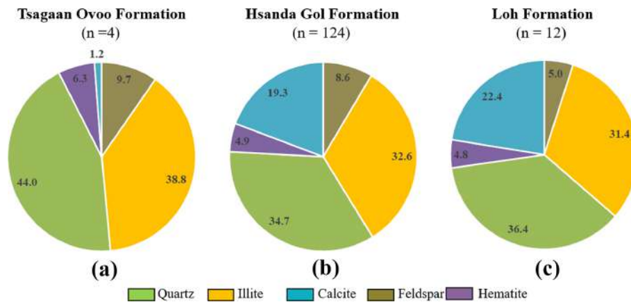
Figure 3. Averaged mineralogical composition (in wt%) of the sediments from the (a) upper-Eocene Tsagaan Ovoo Formation, (b) Oligocene Hsanda Gol Formation and (c) lower-Miocene Loh Formation from the Valley of Lakes, determined by XRD analysis.
