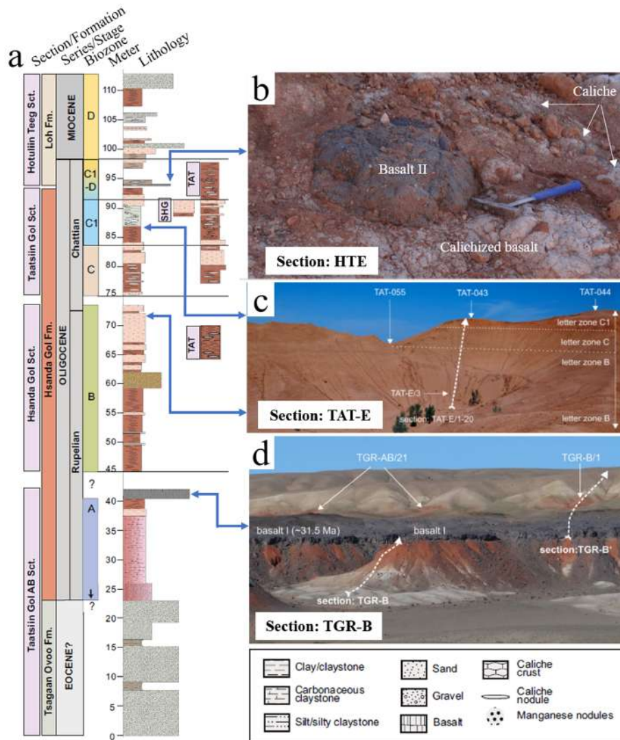
Figure 2. (a) Integrated lithostratigraphic profile of the investigated sedimentary succession from the Taatsiin Gol region, Valley of Lakes (modified after Richoz et al., 2017), with biozonation (modified after Harzhauser et al., 2017). (b–d) Field impressions of the sections: Hotuliin Teeg (HTE) with the calichized basalt II group, Tatal Gol (TAT-E) sediments and the Taatsiin Gol right (TGR-B) section with the basalt I group (modified after Daxner-Höck et al., 2017).
