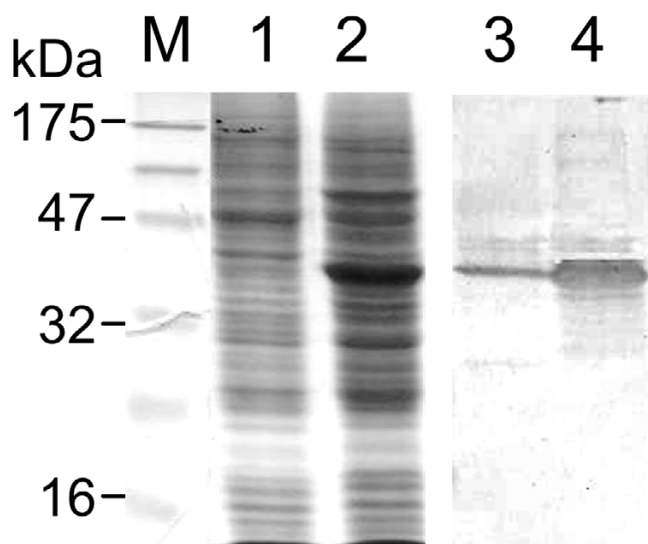
Figure 1 SDS-PAGE and immunoblot analysis of rHA1 protein expressed in a baculovirus/insect cell system under monolayer (lanes 1 and 3) and suspension (lanes 2 and 4) culture conditions. Values on the left indicate molecular weights of the marker protein (lane M). The rHA1 was detected by immunoblotting with rabbit anti-H5N1 serum.
