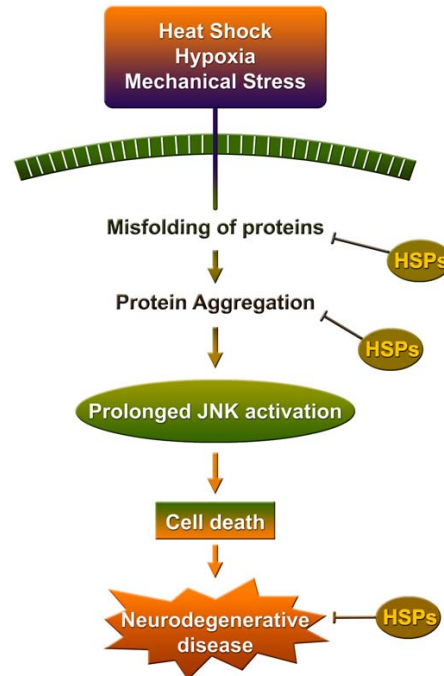
FIGURE 1. Misfolded proteins and neurodegenerative disorders. External stresses, such as heat shock, hypoxia, and mechanical stress, induce the production of reactive oxygen species and denaturation of cellular proteins. Moderated stress on the cell system induces HSP expression. These HSPs are capable of ensuring proper folding or treatment of misfolded proteins, as well as inhibiting protein aggregation, thus preventing neurodegenerative diseases that result from high stress-induced cell death[29].
