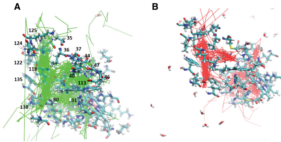
Figure 4. A. F97L trajectories highlighting the internal cavities. B. F07V trajectories highlighting the internal cavities. The internal cavities in each structure can be compared with the B, Xe4, Xe2, and Xe1 cavities shown in Figure 2B .
