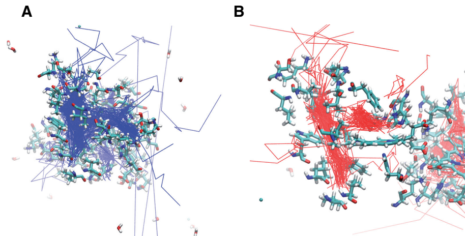
Figure 5. A. M37V trajectories showing the internal cavities used for oxygen escape. B. M37F trajectories reveal the internal cavities for ligand transport. The relative position of each internal cavity can be compared to the B, Xe4, Xe2, and Xe1 cavities in Figure 2B .
