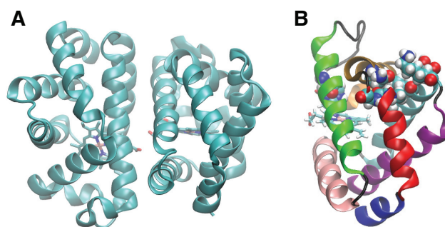
Figure 1. A. Crystal structure of HbI obtained from the protein data bank (ID: 3SDH). B. The helices of HbI are colored as follows: A-blue, B-red, C-ochre, D-orange, E-green, F-pink, G-cyan and H-purple. The residues shown in space-filling representation were found by implicit ligand sampling 10 to be on the major ligand escape. His69 is at the subunit interface on the E alpha helix, and the rest of the residues form a channel between the B and G helices; including Ile25, Asn32, Ala35, Leu36, Val121, Ser124, and Lys125. The E and F helices are involved in intra-subunit communication. The BG pathway is adjacent to the Xe4 cavity ( Figure 2B ), allowing escape between these two helices.
