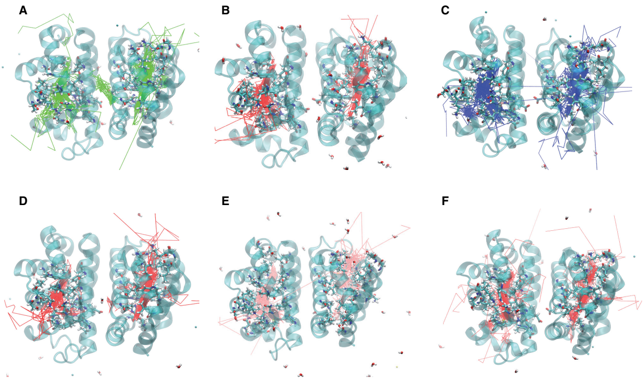
Figure 3. The oxygen trajectories are displayed for all 14 oxygen molecules in the six mutants studied. The trajectory for a particular oxygen molecule was recorded until it escaped the protein, “escape” being defined as more than 5 Å from the protein surface. The trajectories for oxygen molecules that failed to escape were recorded for the entire 10 ns. A. F97L B. F97V C. M37V D. M37F E. I114F F. I25W.
