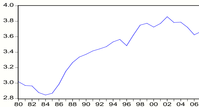
Figure 4. Sigma Convergence
