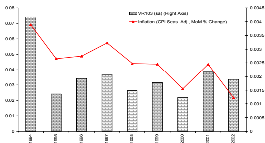
a.) Yearly Averages (1994:02-2002:12)
