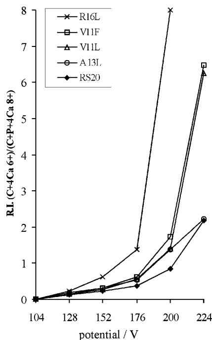
FIGURE 10 Stability in the gas-phase of the CaM-peptide-Ca 4 complexes shown as a function of capillary potential. The ratio was calculated using the relative intensities of signals corresponding to CaM-peptide-Ca 4 complex at the 8 + charge-state and CaM-Ca 4 at the 6 + charge-state. C represents CaM and P peptide, respectively.
