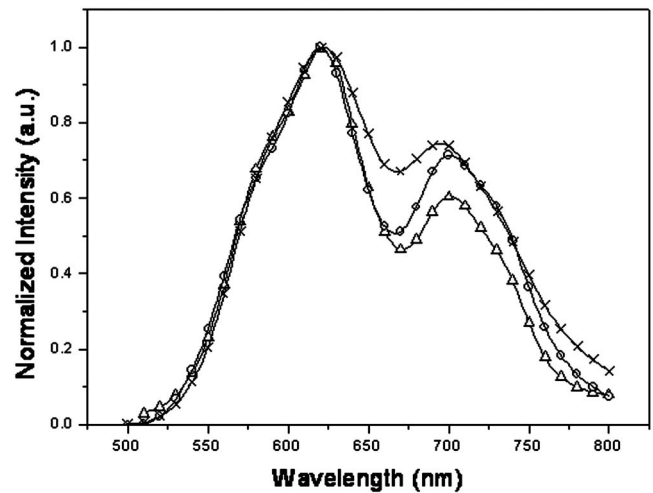
FIG. 2. Electronic absorption spectra of a 300 Å CuPc layer grown directly on ITO (crosses) and on a 20 Å PTCDA interlayer (empty circles), and a 1000 Å CuPc layer grown on a 20 Å PTCDA interlayer (empty triangles).
