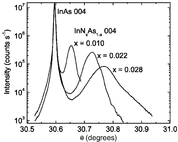
FIG. 1. X-ray diffraction of the 004 Bragg peaks from nominally 300-nm-thick InAs epilayers MBE-grown on InAs(001) substrates, indicating N contents of 1.0%, 2.2%, and 2.8%.
