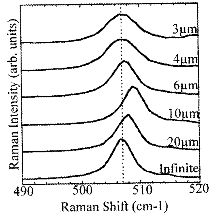
FIG. 5. Si-Si Raman frequency shift as a function of lateral dimension of the uniform \text{Si}_{0.77}\text{Ge}_{0.23} epilayer deposited on the linearly graded buffers. The dashed line corresponds to \sim 80\% relaxation whilst the residual strain within the 10 \mu\text{m} deposition indicates \sim 50\% relaxation.
