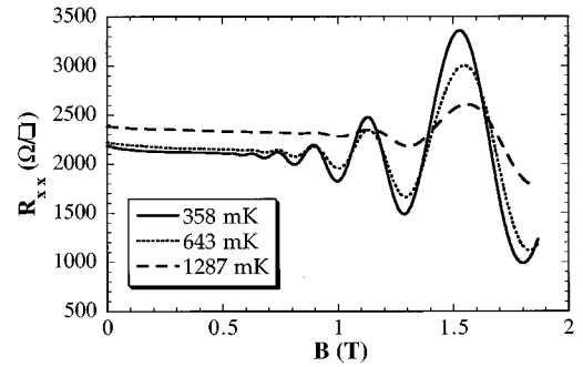
FIG. 3. The reduction of the amplitude of the Shubnikov–de Haas oscillations as the temperature was increased is demonstrated by plotting three different temperatures. The small change in hole density with temperature can be observed by the movement of each peak to higher B as the temperature increases.
