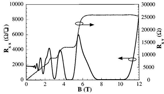
FIG. 2. The longitudinal and transverse resistivity of the 2DHG SOI wafer as a function of transverse magnetic field. The temperature was 298 mK and the mobility and sheet carrier density measured were 16\,810\text{ cm}^2/\text{Vs} and 2.05 \times 10^{11}\text{ cm}^{-2}/\text{V s} , respectively.
