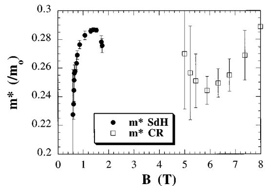
FIG. 4. The effective masses (in units of free electron mass, m_0 ) obtained from the temperature dependence of the Shubnikov–de Haas oscillations (solid circles) and the cyclotron resonance (open squares) measurements.
