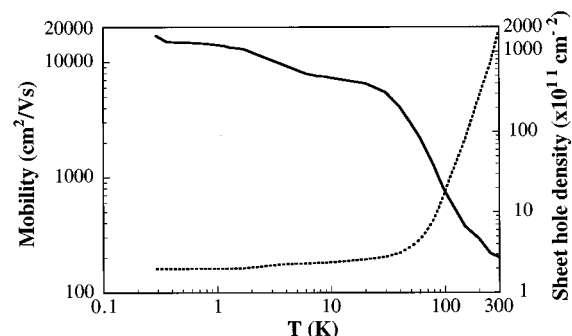
FIG. 1. The mobility (solid line) and sheet hole density (dashed line) as a function of temperature.
