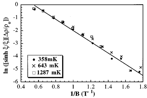
FIG. 5. Dingle plots for three temperatures.
