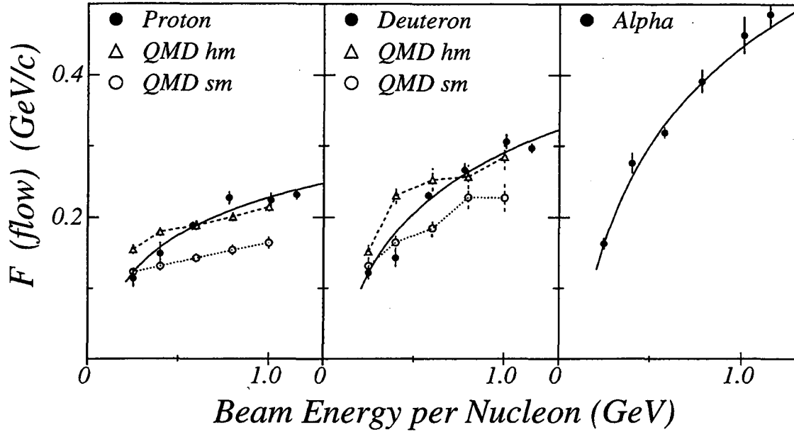
FIG. 3. Directed collective flow, F , for different fragment species and QMD model calculations using a hard equation of state with momentum dependent interactions (hm) and a soft equation of state with momentum dependent interactions (sm).
