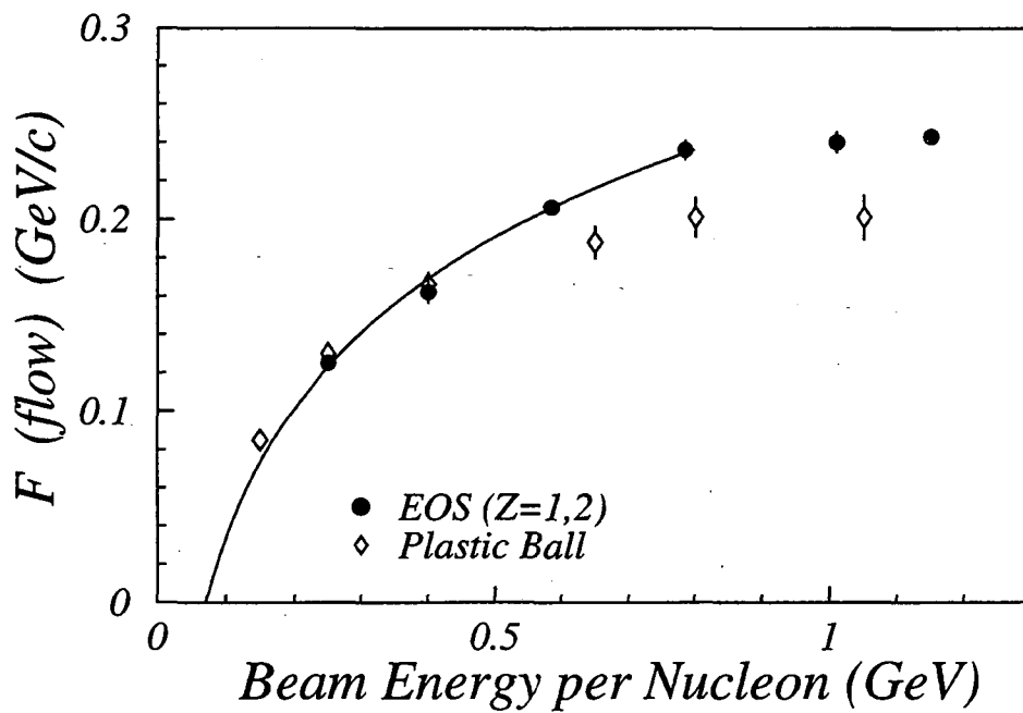
FIG. 2. Energy dependence of flow from EOS data and Plastic Ball data of Ref. [13].
