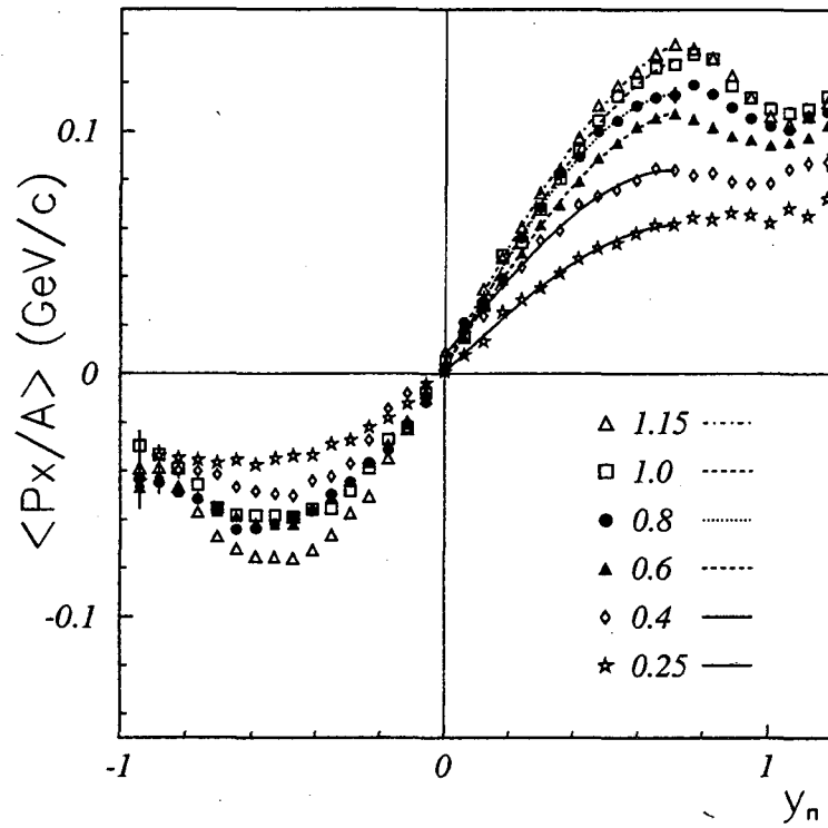
FIG. 1. \langle P_x/A \rangle vs y_n for each beam energy. The data are from events in multiplicity bins 3 and 4. The fragments included are p, d, t, ^3\text{He} , ^4\text{He} . The curves are fits to the data and indicate the region in which the fits were made.
