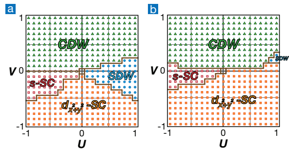
FIG. 2: (Color online) The phase diagram (a) at half-filling \mu = 0 , (b) at \mu = -0.095 , parameterized by on-site U and nearest-neighbor interaction V . The interaction terms U and V are in units of t throughout this paper.
