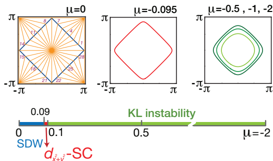
FIG. 1: (Color online) Fermi surfaces of a square lattice with nearest-neighbor hopping, at different chemical potentials \mu (in units of t ). Below, the phase diagram versus \mu for U = 1 and V = 0 . The Fermi surface patches used in this study are illustrated in the Fermi surface at \mu = 0 .
