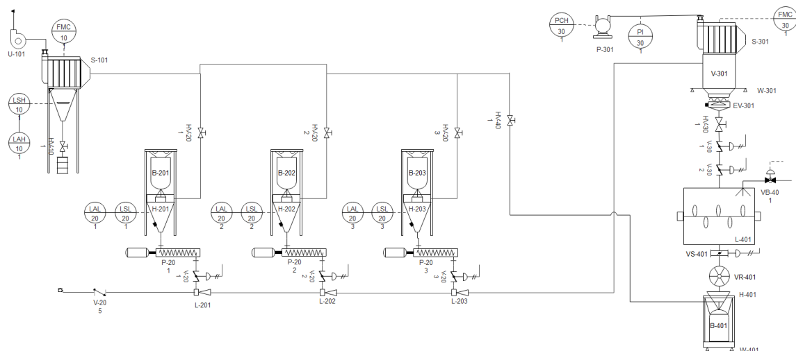
Figure 1: P&ID for the plant processing the stearate
