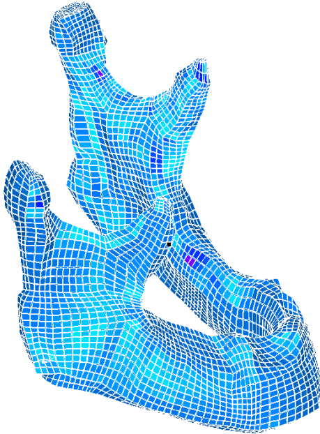
Figure 11: A refinement of the hexahedral mesh in Fig. 9 with 18674 hexahedra.
