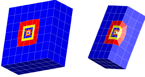
Figure 8: Example: Insertion of internal sheets.
