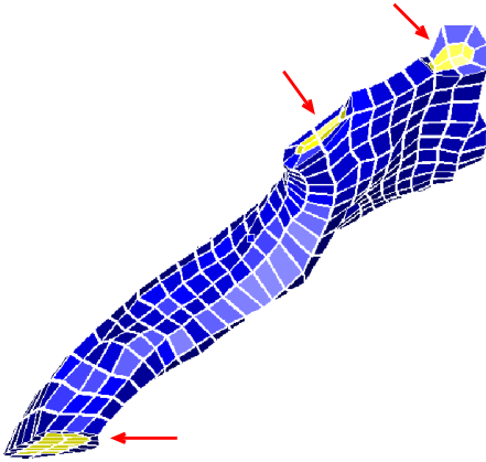
Figure 6: Example: Three-step-elimination (arrows point to the three selected dual cycles).
