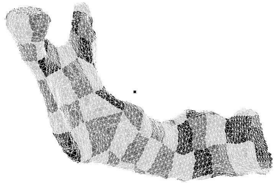
Figure 3: The clustering of one half of the mandible into multi-patches.
