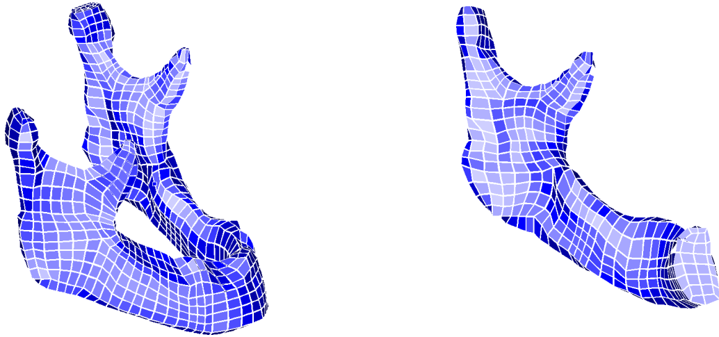
Figure 9: Hexahedral mesh for the mandible with 2252 elements (left), and one part of it after a split (right).
