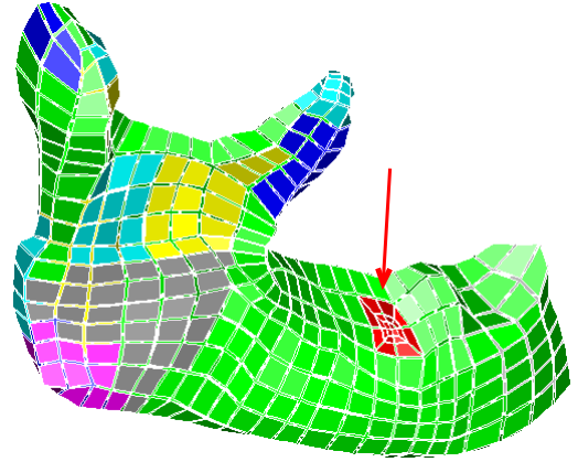
Figure 7: Local mesh refinement at the biting point (indicated by the arrow).
