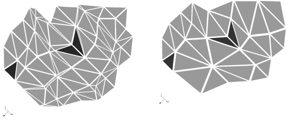
Figure 2: Removal of extreme triangles by iterated edge contractions.
