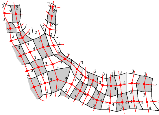
Figure 5: The b -matching problem defined on the dual graph of the coarse multi-patch quadrangulation, the given numbers attached to the edges are the b -matching values and denote the number of dual cycles crossing each primal edge (left), and the embedding without self-intersections of the b -matching decomposition into dual cycles (right).
