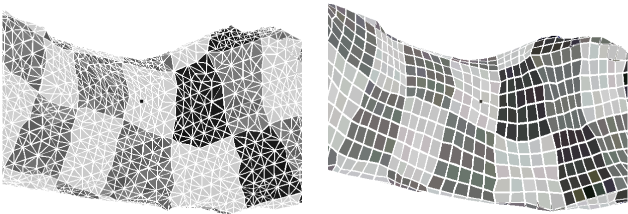
Figure 4: A detailed view on the multi-patches.
