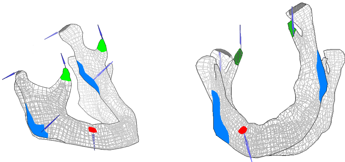
Figure 13: Deformation of the mandible (100 times exaggerated, order of magnitude 5.0 \cdot 10^{-5}m ) occurring at a lateral bite: the colors show the placement of the masticatory muscles and the biting point. The arrows indicate the assumed muscle forces.
