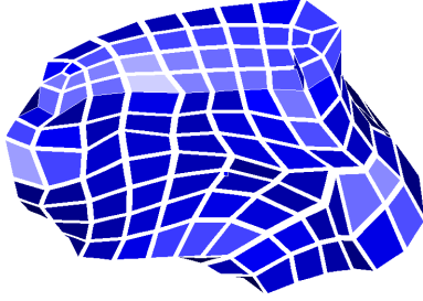
Figure 10: Part of the hexahedral mesh for the mandible.
