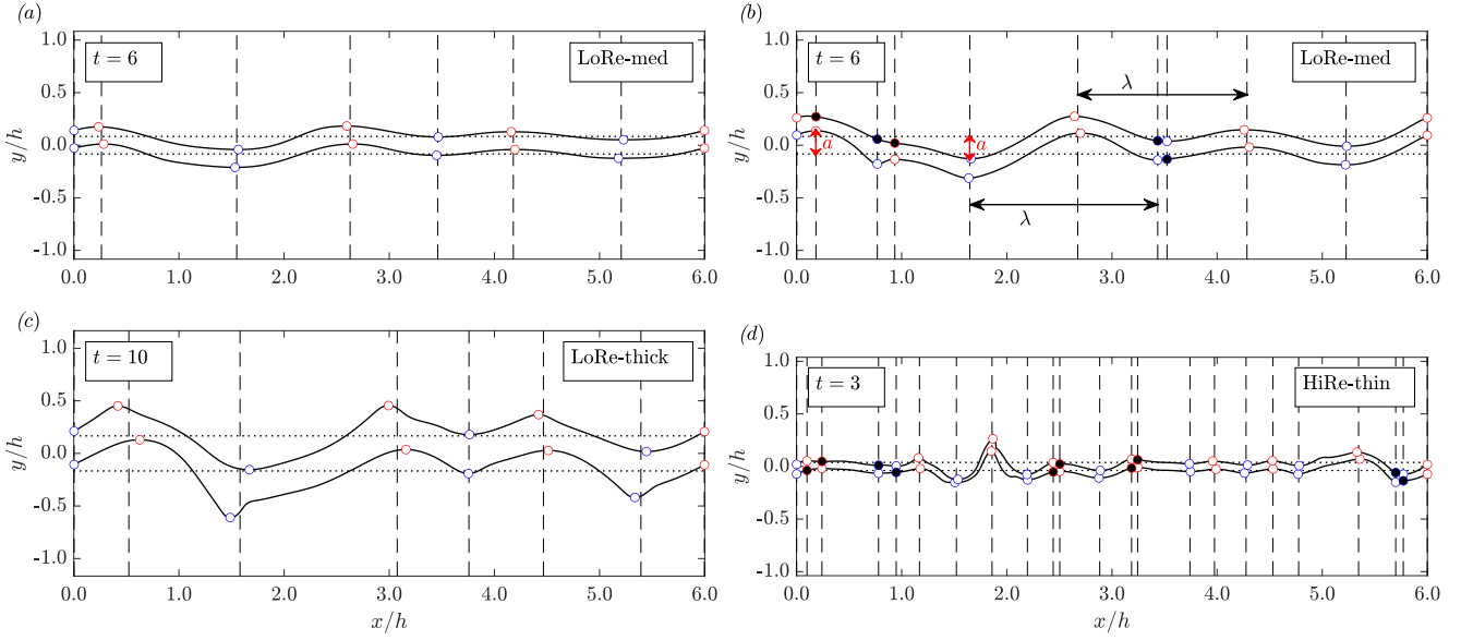
FIG. 8. Indicative division of the deforming film into segments or panels, indicated by the vertical dashed lines, based on local minima and maxima (open bullets); (a,b) samples from the LoRe-med case at t = 6 at two different spanwise locations; (c) LoRe-thick case at t = 10 ; (d) HiRe-thin case at t = 3 . Filled bullets indicate points added from one side of the film to another if absent within a specified tolerance based on the starting film thickness. This procedure is carried out for each spanwise grid location. In some cases (e.g. subfigures (a) and (c)) no additional points need to be added, but in most cases (e.g. subfigures (b) and (d)) they are required in order to deduce the panel segments for the calculation of C_{L,cumul.} . For the purposes of calculating wavelengths ( \lambda ) and amplitudes ( a ) of the deforming liquid surface, only genuine local extrema (open bullets) are used; sample measurements marked in (b).
