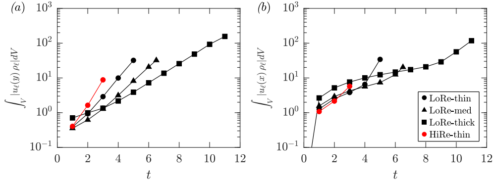
FIG. 15. Impulse on the liquid film over time (change in momentum); (a) film-normal impulse; (b) streamwise impulse. Symbols as per legend in (b).
