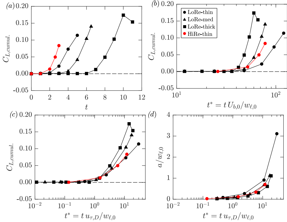
FIG. 13. (a) Cumulative Lift coefficient C_{L,cumul.} (same as figure 12a); (b) temporal development of C_{L,cumul.} scaled with t^* formed from the starting bulk velocity U_{b,0} and the starting film thickness w_{l,0} ; (c) temporal development of C_{L,cumul.} scaled with t^* formed from u_{\tau,D} , a friction velocity derived from the lift-induced drag force F_{D,p} and w_{l,0} ; (d) amplitude of film deformation scaled with w_{l,0} , measured as a deviation from the original film surface location (figure 9b), plotted against the scaled time t^* formed from u_{\tau,D} and w_{l,0} as in (c). Symbols as per legend in (b).
