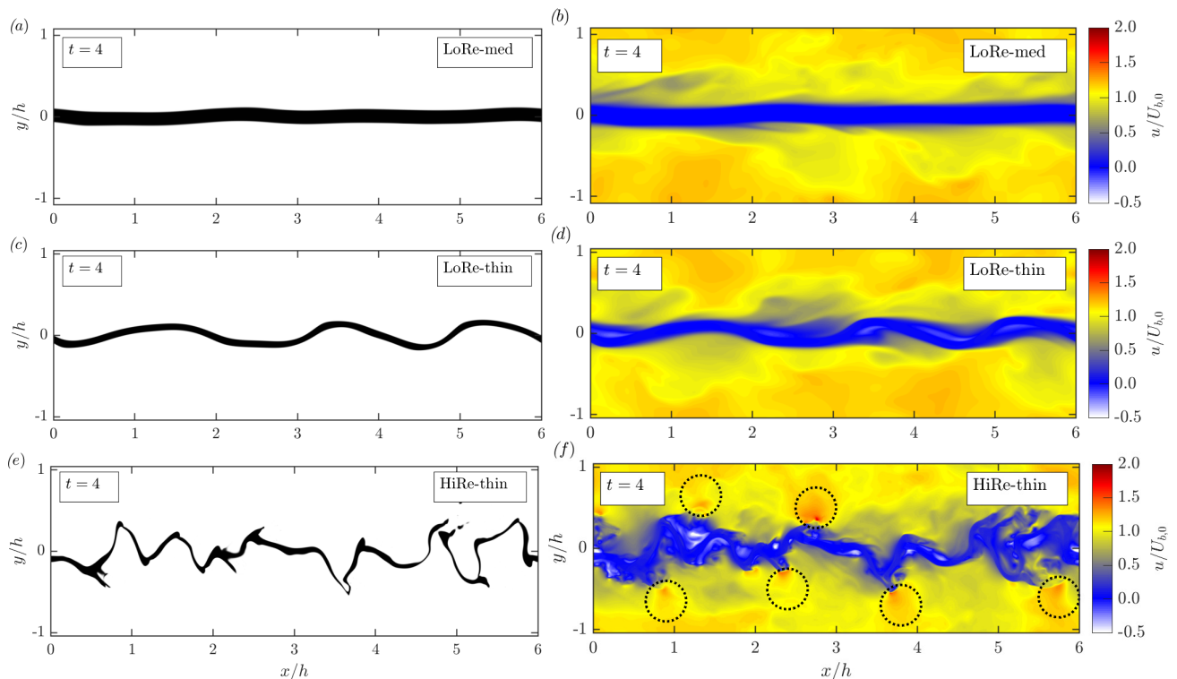
FIG. 4. Visualisations of three cases of the VoF simulations at t = 4 . Top, LoRe-med case; middle, LoRe-thin case; bottom, HiRe-thin case. Left, the cell-averaged volume fraction of the liquid, \phi ; right, streamwise velocity fields. Dotted circles in (f) mark regions of high streamwise velocity. Bulk velocity is to the right.
