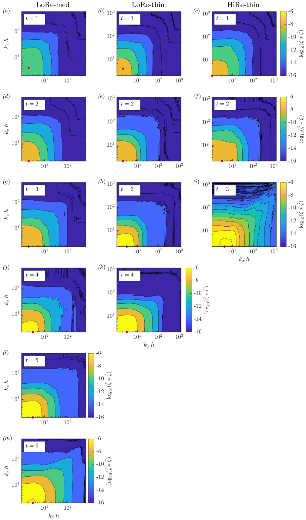
FIG. 7. Spectra of the surface displacement \zeta , computed for the same top film surfaces for the same three cases shown in figure 6. The maximum in each subfigure is marked with a red bullet.
