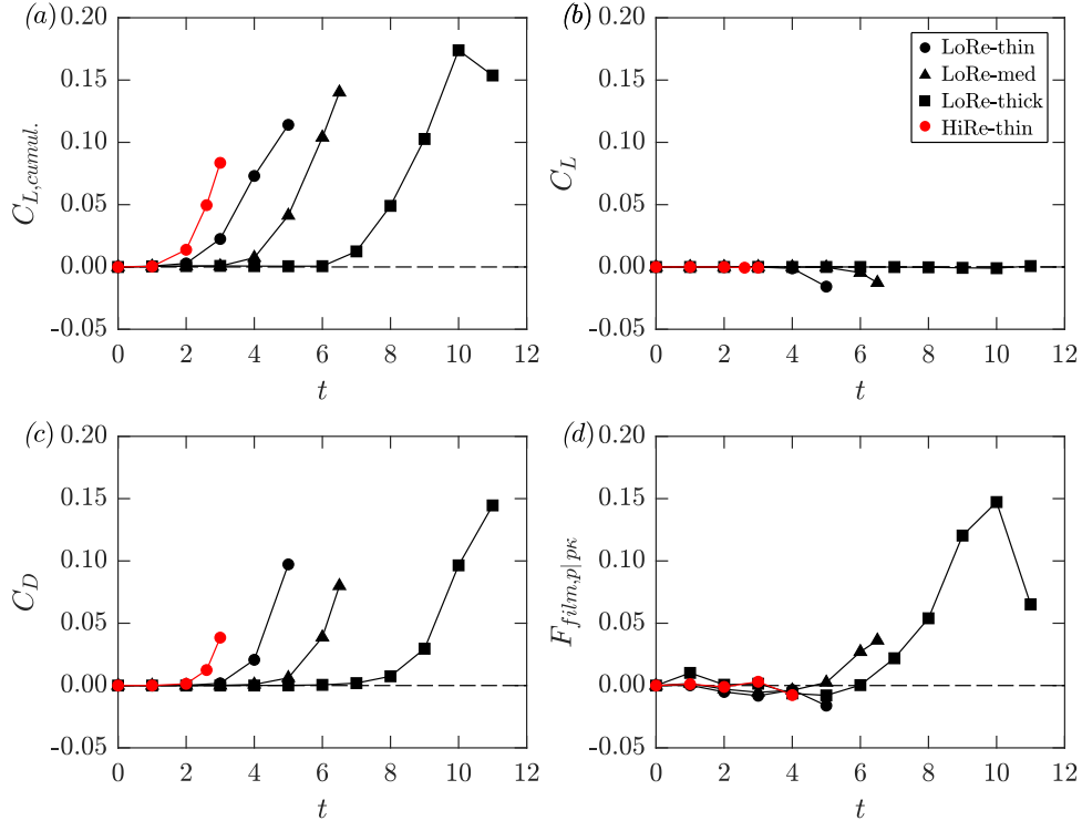
FIG. 12. Aerodynamic coefficients over the deforming film for the different cases. Symbols as per legend in (b).
