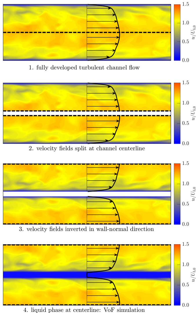
FIG. 1. Four-step method to set up the VoF simulations: use of velocity fields from fully developed turbulent channel flow simulations. Shown here are contours of the streamwise velocity however the procedure is applied to all three velocity components to form the starting fields of the VoF simulations. Thick black contour indicates the initial mean streamwise velocity profile. Dashed lines indicate how a single plane at the centerline is recast as a periodic boundary condition, meaning the flow field is still numerically contiguous in the ‘sandwich’ VoF setup.
