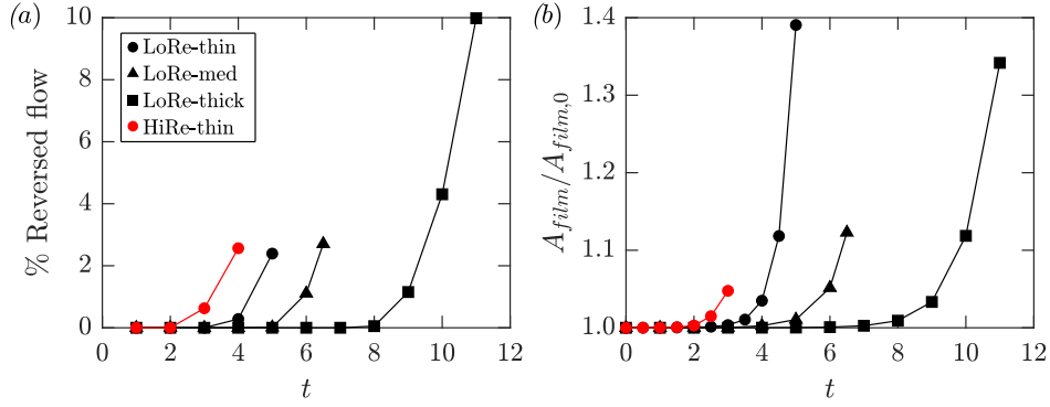
FIG. 14. (a) Percentage of reversed flow in time; (b) increasing total film surface area with time. Symbols as per legend in (a).
