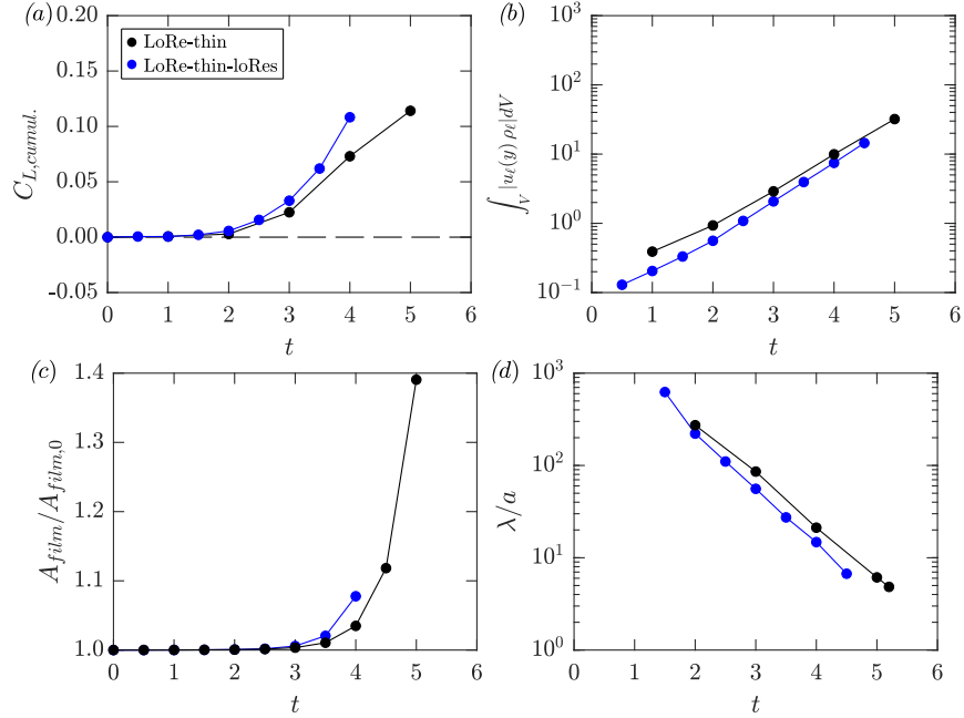
FIG. 17. Comparing the temporal development of bulk quantities for the thin film at two different simulation grid resolutions. Symbols as per legend in (a).
