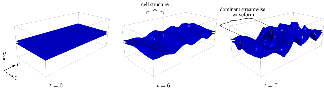
FIG. 2. Visualisation of the surface of the liquid film (contours drawn at \phi = 0.5 ) for the LoRe-med case in time. The initially flat film deforms under the action of the fully developed turbulent gas-phase boundary layers.
