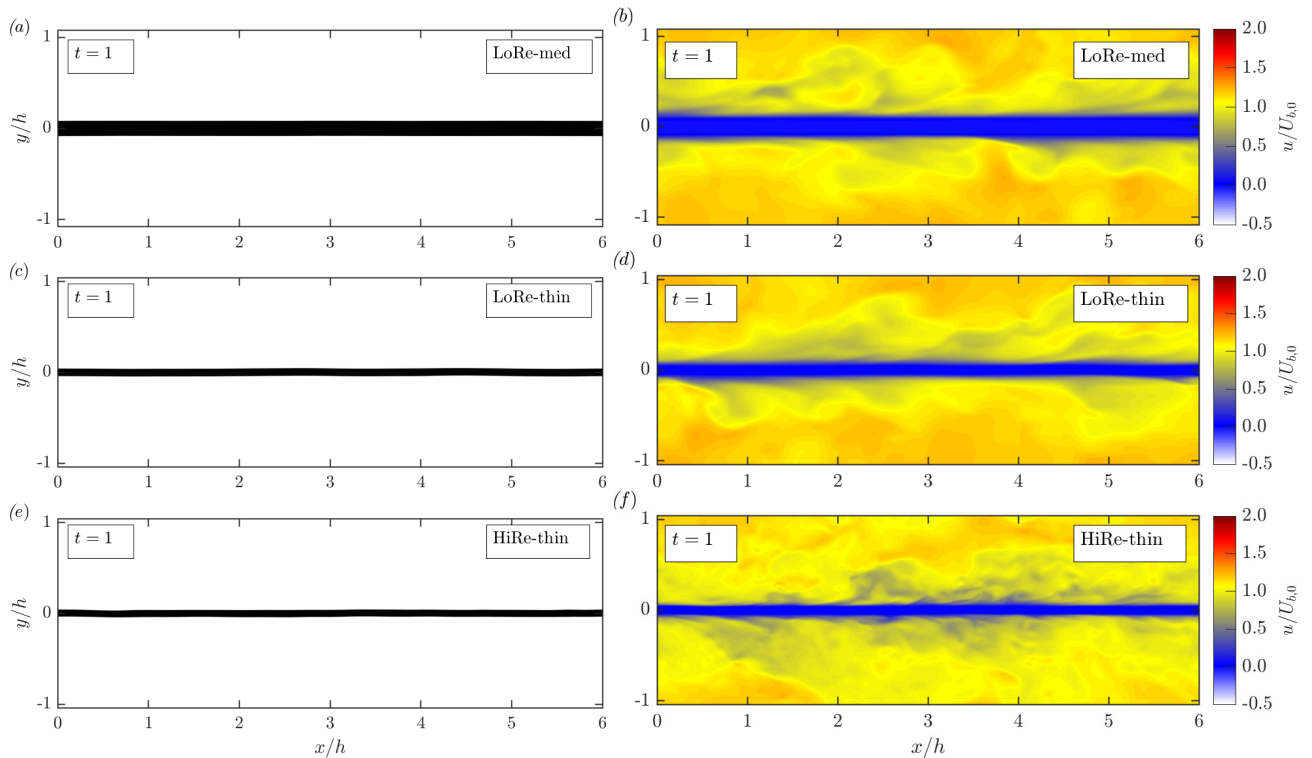
FIG. 3. Visualisations of three cases of the VoF simulations at t = 1 , fields of the ‘sandwich’ film setup at an early time. Top, LoRe-med case; middle, LoRe-thin case; bottom, HiRe-thin case. Left, the cell-averaged volume fraction of the liquid, \phi ; right, streamwise velocity fields. Bulk velocity is to the right.
