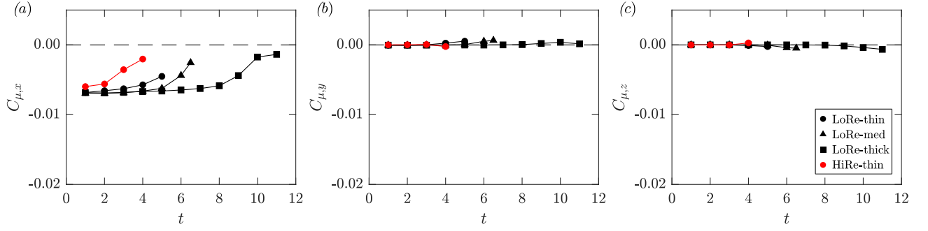
FIG. 11. Viscous stress over the deforming film plotted as skin friction drag coefficients, analogous to figure 12 (note the extent of the vertical axis of these plots is only 1/10th that of the plots in figure 12); (a) streamwise x component; (b) film-normal y component; (c) spanwise z component. Symbols as per legend in (c).
