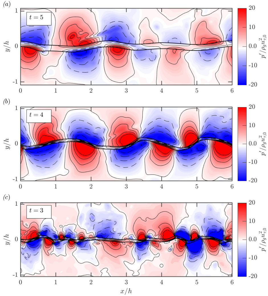
FIG. 10. Indicative contours of the normalised pressure fluctuations over the deforming film for the different cases, contours are spaced at intervals of 5 p' / \rho_g u_{\tau,0}^2 : (a) LoRe-med case, with Re_{\tau,0} = 180 , t = 5 ; (b) LoRe-thin case with Re_{\tau,0} = 180 , t = 4 ; (c) HiRe-thin case with Re_{\tau,0} = 393 , t = 3 . Solid lines denote positive contours and dashed lines negative contours in each case. Thicker black contours denote the surface of the liquid film.
