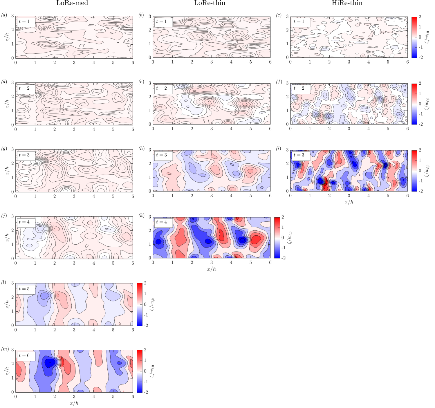
FIG. 6. Contours of the deforming (top) film surface displacement \zeta for the same three cases shown in figures 3, 4 and 5, scaled by initial film thickness w_{\ell,0} . Time advances downward in each column for each case. Contours are similar for the bottom film surface (not shown).
