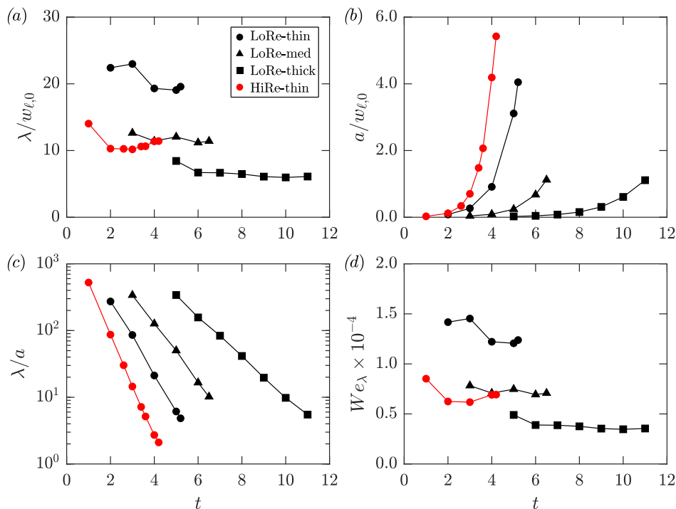
FIG. 9. Characteristics of the deforming film as a function of time; (a) streamwise wavelength of the film’s surface \lambda ; amplitude of surface deformation a (measured as the difference from the original film’s location on either side); (c) ratio \lambda/a ; (d) We_\lambda , a Weber number defined using \lambda , the streamwise wavelength of the deforming film. Note that significant film deformation must occur to reliably measure of \lambda or a , therefore the curves in figure 9 begin at different t \geq 1 depending on the film’s rate of deformation. Symbols as per legend in (a).
