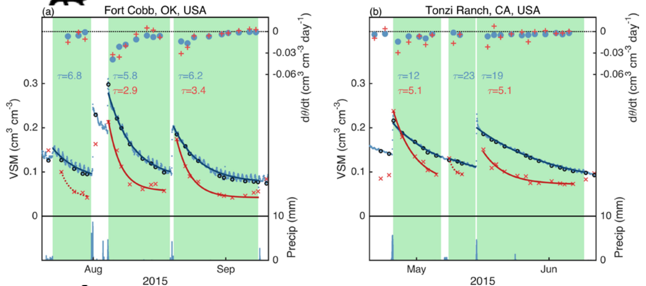
Figure 1. Rainfall (bottom), volumetric soil moisture (VSM; middle), and soil drying rates (top) at Fort Cobb, Oklahoma (a) and Tonzi Ranch, California (b). Drydowns are highlighted in green.
