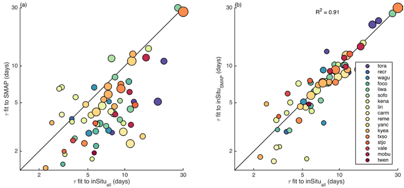
Figure 2. (a) Relationship between inSitu all -fit and SMAP-fit \tau values. (b) Relationship between inSitu all -fit and inSitu SMAP -fit \tau values. Marker colors correspond to each site as shown. Marker sizes correspond to length of drydown.
