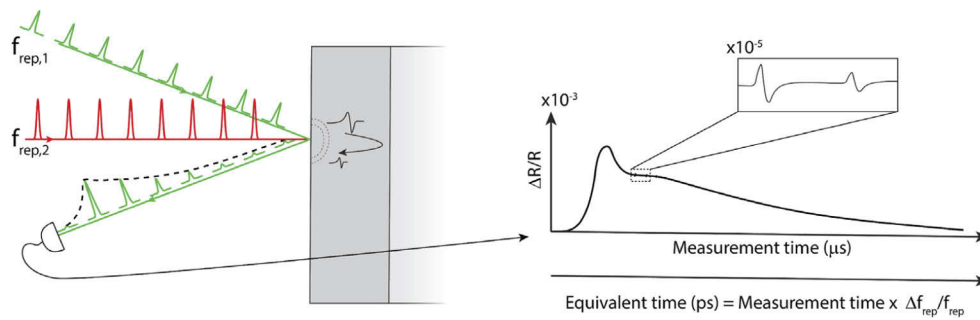
Fig. 1. Schematic illustration of a picosecond ultrasonics measurement with the pump and probe having two slightly different repetition rates f_{\text{rep},1} and f_{\text{rep},2} . The pump (red) excites an ultrasonic wave in a sample. The returning reflection is then sampled with the probe (green). The signal is detected with a photodiode and recorded on an oscilloscope (right). Within the timescale of the thermal response of the sample, ultrasonic signatures can be observed (inset). The measurement time is related to the equivalent pump-probe time by the laser repetition rate difference and probe repetition rate ratio.
