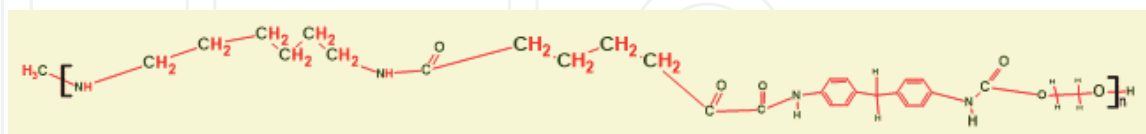
Figure 7. Coupling of TPU-DMF treated PA-6,6.
