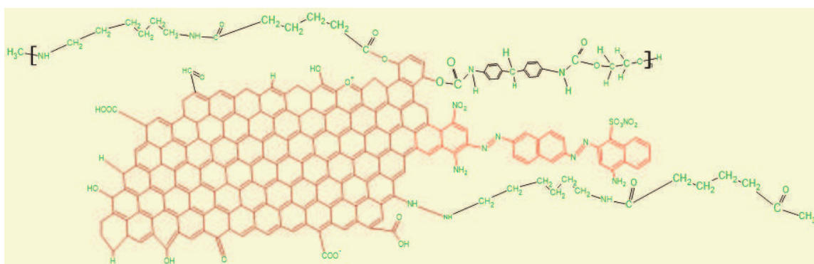
Figure 10. Coupling of CBP-TVR- TPU-DMF treated PA-6,6.
