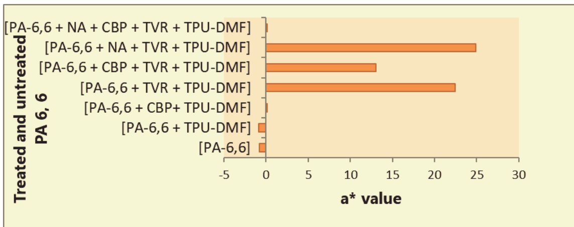
Figure 14. CIE comparison of greenish/reddish hue ( a^* ) of treated and untreated PA-6,6 fabric.
