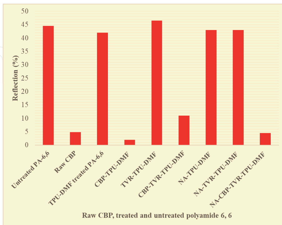
Figure 17. Comparison of maximum reflection (%) in NIR spectrum.
