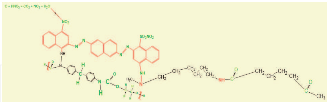
Figure 11. Coupling of NA-TVR-TPU-DMF treated PA-6,6.
