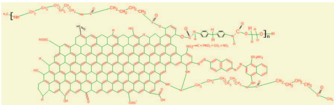
Figure 12. Coupling of NA-CBP-TVR-TPU-DMF treated PA-6,6.
