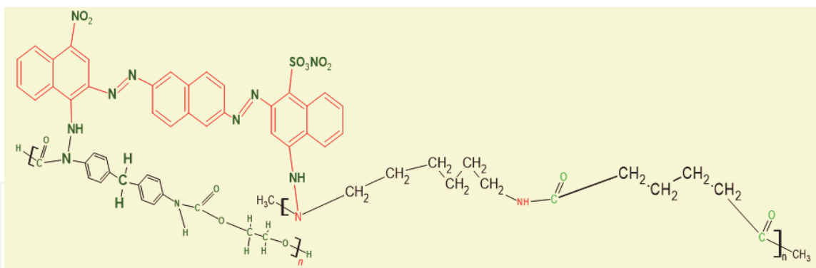
Figure 9. Coupling of TVR-TPU-DMF treated PA-6,6.
