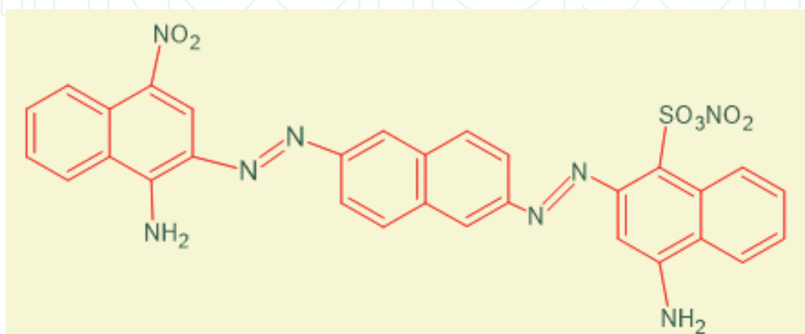
Figure 2. Structure of TVR used in this experimentation.
