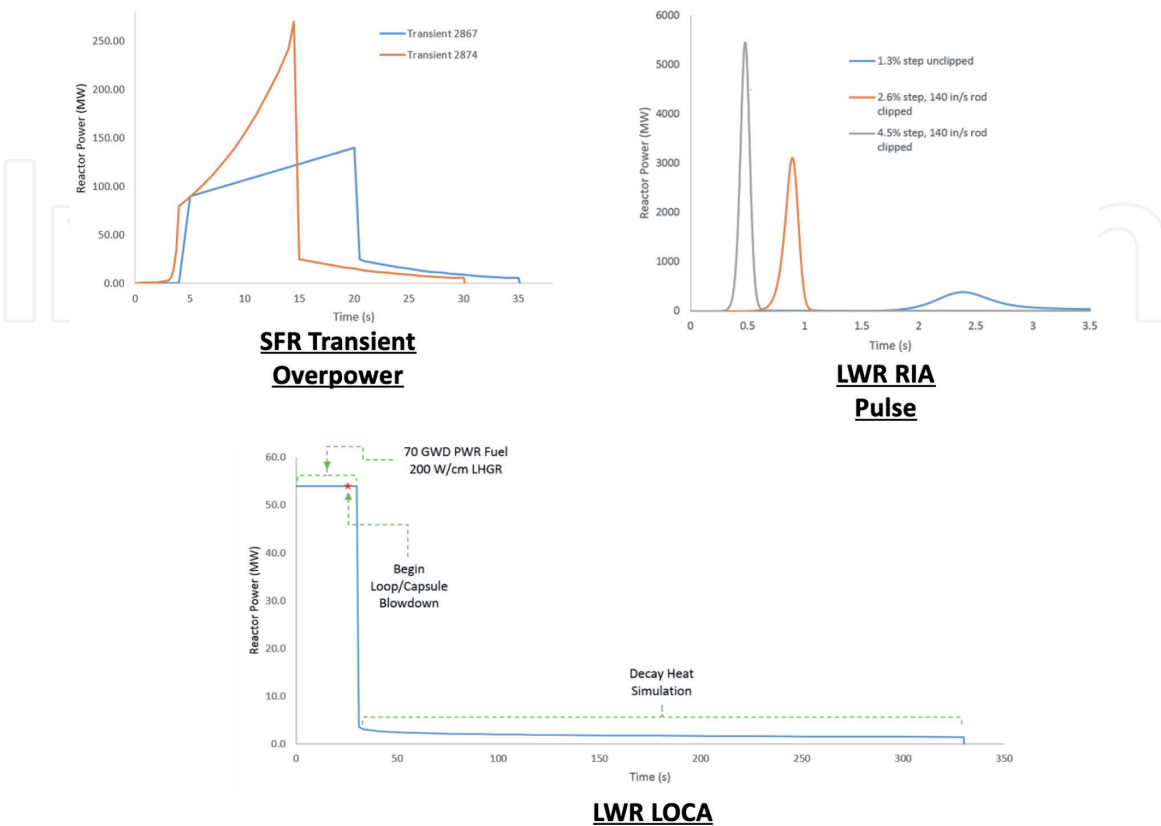
Figure 7. Example transient shapes possible at TREAT.
