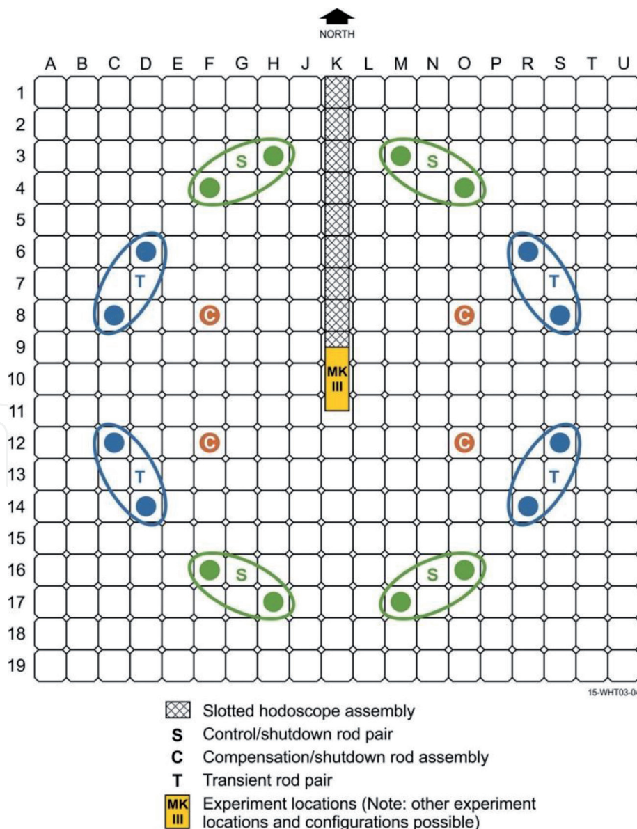
Figure 5. Example core map showing current control rod types and locations.
