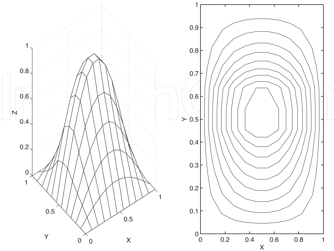
Figure 2. Approximate solution u_h^{(0)} .
