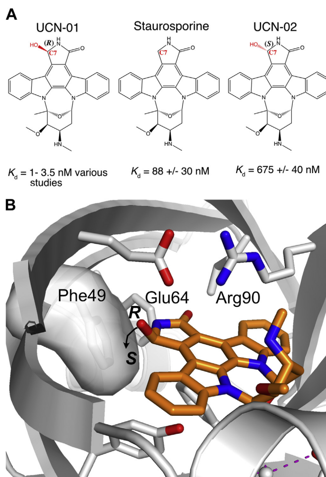
Figure 5. Proposed structural basis for affinity of UCN-01, -02 and staurosporine for AGP2. A, chemical structures of staurosporine and UCN-01 and -02 derivatives showing switch in stereochemistry of the C7 hydroxyl group. B, potential clash with Phe49 (shown in space-filling) when C7 hydroxyl group is in the S -configuration (UCN-02).
