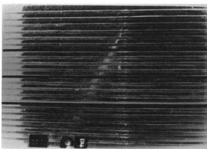
Image of a shower due to interaction of hadron in the Big Multi-plate Cloud Chamber in the experiment at Ooty (Courtesy: J. Acharya, Photography Section, TIFR).
