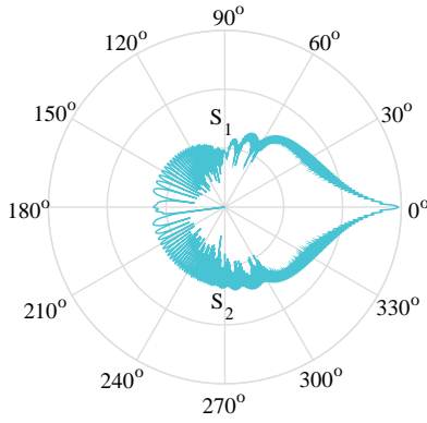
(a) The scattering amplitudes polar plot of S_1 on 0^\circ \leq 180^\circ and S_2 on 180^\circ \leq 360^\circ .
