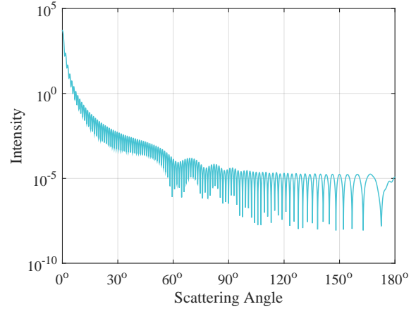
(b) The logarithmic Cartesian plot of light intensity as a function of scattering angle
