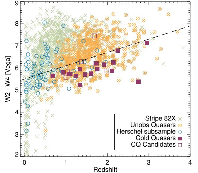
FIG. 7.— We show the slope of the mid-IR emission, parameterized as W2 - W4 , as a function of redshift. Our Cold Quasars (purple squares) have bluer colors than the unobscured quasars in the parent sample (orange circles with crosses). All Cold Quasars lie below W2 - W4 = 0.6z + 5.5 , plotted as the dashed line. The bluer colors may be due to a torus with a small optical depth, patchy circumnuclear dust, or increasing contribution to the mid-IR colors from star-forming regions.
