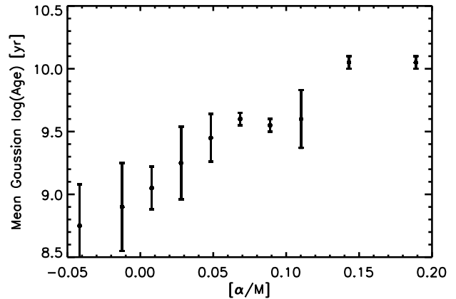
FIG. 14.— The mean \log(\text{age}) , \tau , of the \alpha -dependent Gaussian+uniform SFH models as a function of \alpha -abundance bin. The error bars indicate the dispersion of each Gaussian model. The mean age of the models increases continuously with \alpha -abundance, even at the youngest ( < 1 Gyr) ages.
