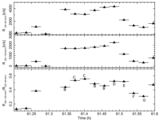
FIG. 2.— Light curves of the major flare in the 25-50 keV (top panel) and 50-100 keV (center panel) bands. Start time is MJD 57190, 21:30:45:186 UT. The hardness ratio in the two bands is shown in the bottom panel. Periods B to G mark the intervals used for the spectral analysis (see text for details).
