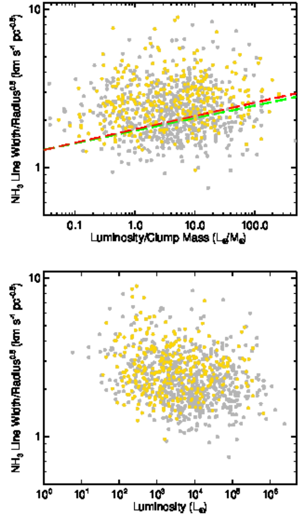
Figure 31. NH 3 (1,1) line-width normalised by the square-root of the clump radius as a function of the L_{\text{bol}}/M_{\text{clump}} ratio (upper panel) and as a function of the bolometric luminosity (lower panel). The grey circles show the distributions of all clumps while the yellow shows the distribution of the distance-limited sample. The distribution in the upper panel is weakly correlated but the distribution in the lower panel is uncorrelated. The long-dashed red and green lines shown in the upper panel shows the result of a linear power-law fit to the whole sample of associated clumps and to the distance-limited sample, respectively.
