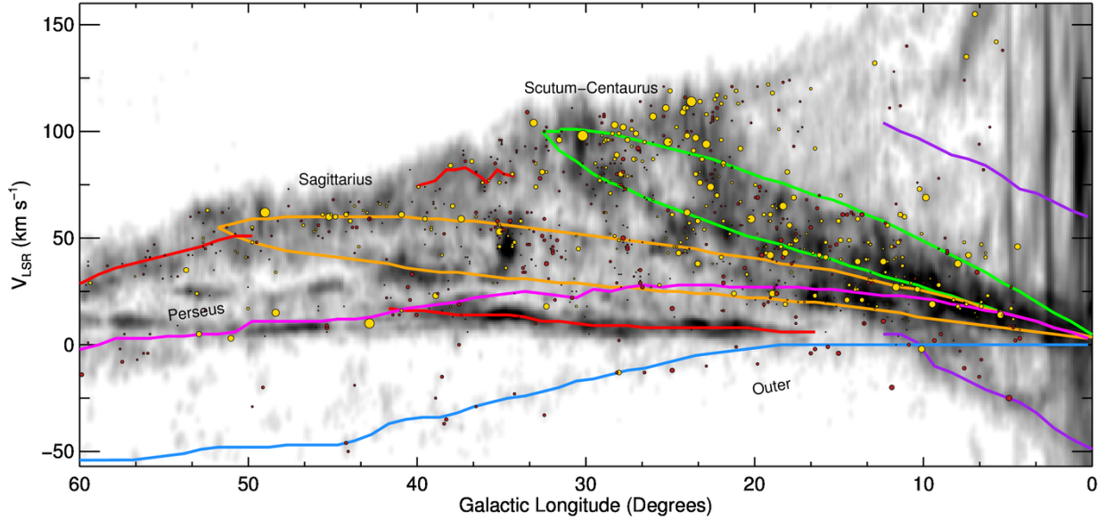
Figure 20. Longitude and velocity ( l-v ) distribution of clumps and complexes located in the first quadrant. The greyscale image is the integrated ^{12}\text{CO} emission from Dame et al. (2001), and the red and yellow circles show the positions of the clumps and clusters, respectively. The sizes of the symbols give an indication of the masses of individual clumps and clusters. This map differs from the one presented in Fig 17 in that the spiral-arm loci are taken from the Reid et al. (2014) model. This map shows the loci of the four main arms (Outer, Scutum-Centaurus, Sagittarius and Perseus, colours are as in Fig. 4), but also includes the near and far 3 kpc arms (lower and upper purple curves, respectively), the local arm (left-most red curve), the Aquila Rift (longest red curve that runs between the Perseus and Outer arms) and the Aquila spur (red curve located between the Sagittarius and Scutum-Centaurus tangents).
