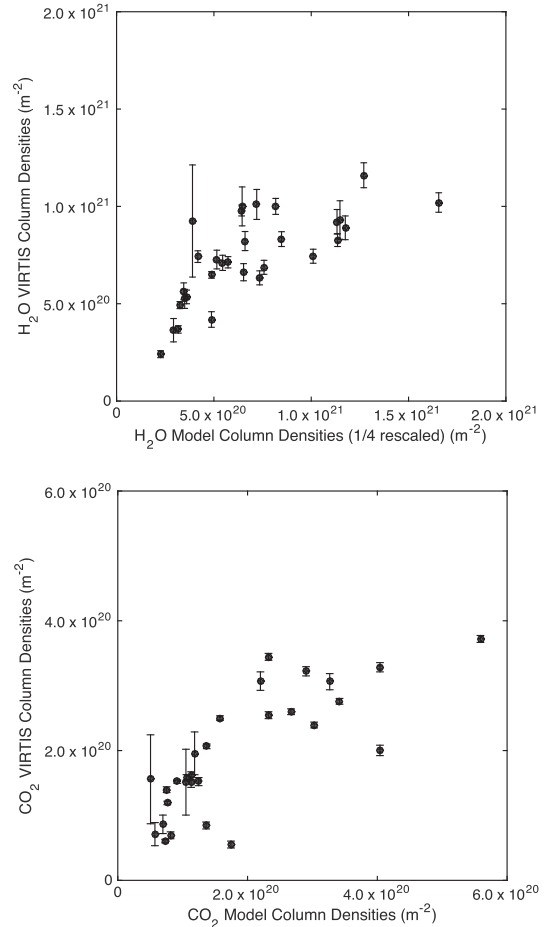
Figure 10. VIRTIS-H column densities deduced from observation times ranging from 2015 July 8 to 2015 September 27 (Bockelée-Morvan et al. 2016) as a function of the model column densities for H 2 O and CO 2 . The model H 2 O column densities were applied a factor of 0.25 to match the data range.
