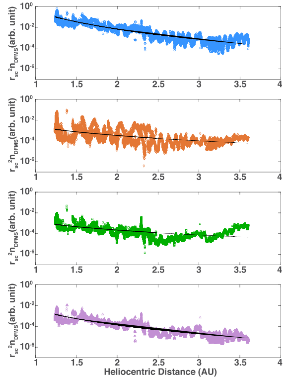
Figure 4. Best fit of the evolution of the number density from DFMS (pre- and post-equinox) times the spacecraft distance squared from the comet in arbitrary units for H 2 O (blue), CO 2 (orange), CO (green), and O 2 (purple) in a function of heliocentric distance, and the corresponding best-fitting power laws with exponents -5.6 , -2.8 , -2.6 , and -4.9 , respectively, which give a priori values for parameter \beta .
