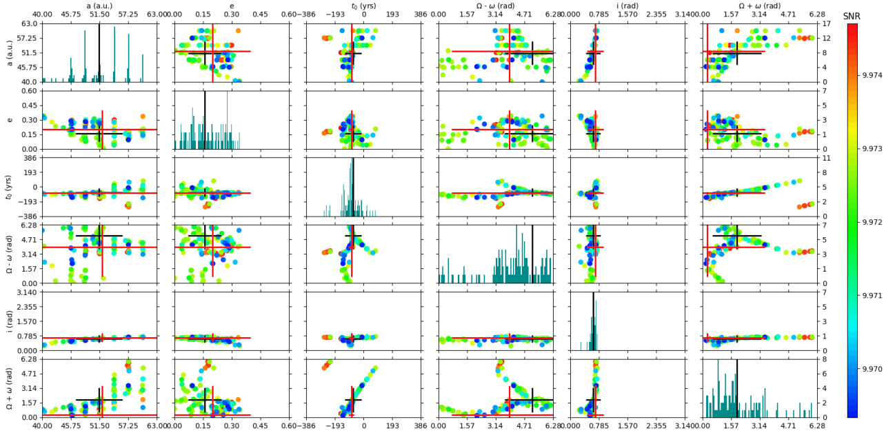
Fig. 10. Histograms and 2D diagrams of the HD 95086 b orbital parameters found by K-Stacker. Left, top, and bottom : scale of the orbital parameters. Right : scale of the histograms. The 129 points in each 2D diagram correspond to the 129 orbits of the higher (S/N)_{\text{KS}} found by K-Stacker. The color of each point gives the (S/N)_{\text{KS}} indicated at right. The dark cross indicates the mean value of the orbital parameters with their error bars. The red cross shows the higher probability density found by an MCMC technique in Chauvin et al. (2018) converted in the K-Stacker referential. The origin of the t_0 K-Stacker date is 05/05/2015.
