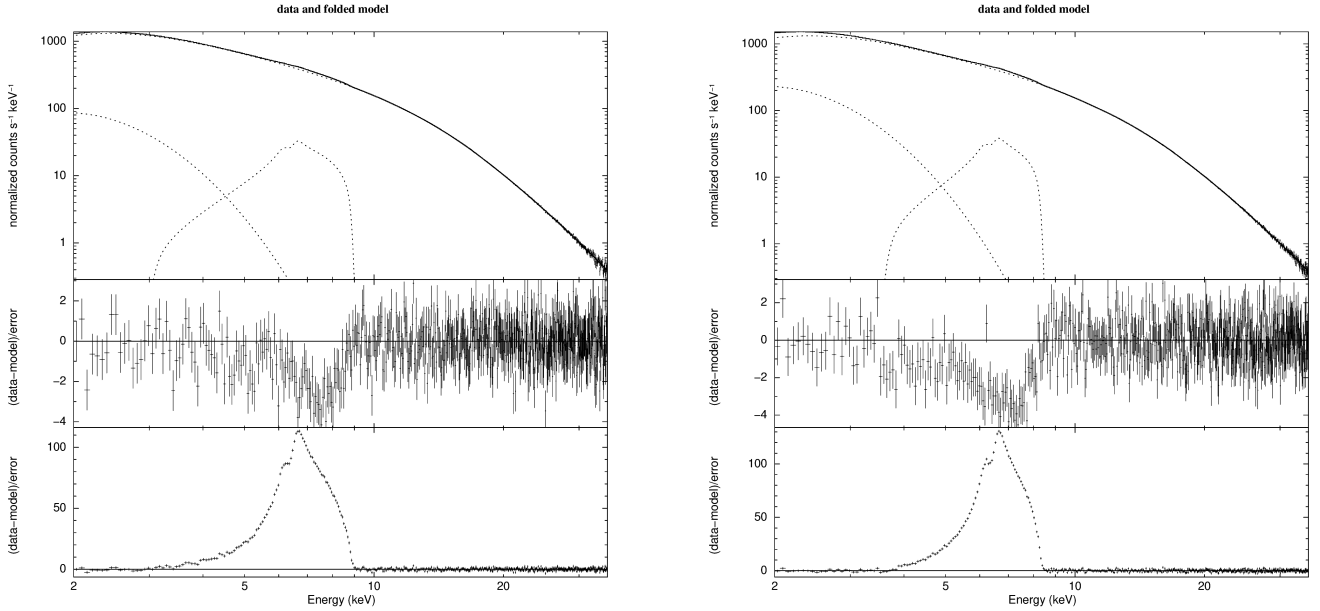
Figure 7. Simulated eXTP spectra from a 100 ks observation of a \sim 120 mCrab system with (left) R_{NS} = 6 r_g , r_{in} = 6 r_g , and i = 80^\circ and (right) R_{NS} = 8 r_g , r_{in} = 8 r_g , i = 75^\circ : in the two middle panels R_{NS} was set to 4 r_g , so the residuals correspond to the deviation produced by not accounting for the occultation; the bottom ones show the residuals with respect to the continuum alone, so that the missing iron line stands out clearly.
