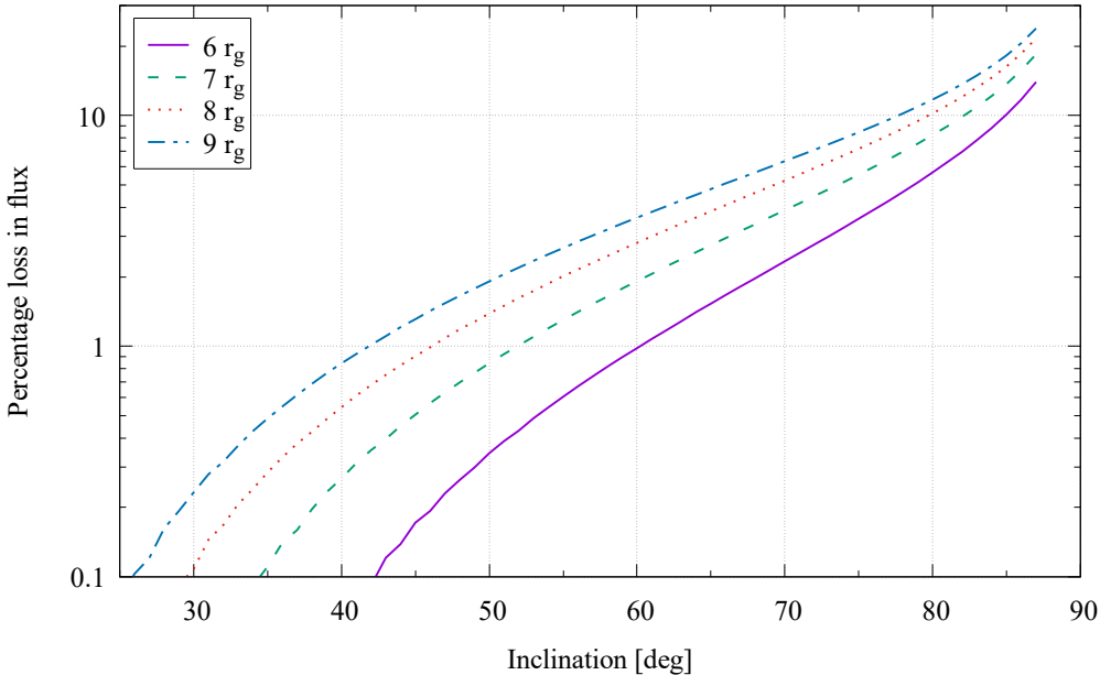
Figure 4. The percentage loss in total flux with respect to the unocculted case is plotted here for different star radii: we used q = -3 and the limb-brightening law, and the disc radii were set to r_{in} = R_{NS} , r_{out} = 5 \cdot 10^5 r_g .
