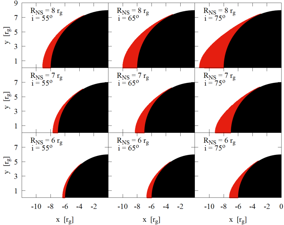
Figure 3. The nine panels show the extent of the occulted area (red) on discs that reach the neutron star (black), for different inclinations and star radii; the observers lie at infinity on the right, on the xz plane, so that the quadrants show half of the “back” side of the star relative to them ( 90^\circ \leq \varphi_{em} \leq 180^\circ ).
