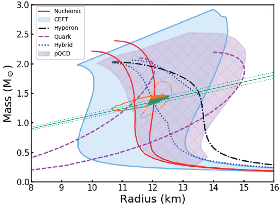
Figure 8. Limits on the mass-radius plane obtained with shaddisk if an R_{NS}/r_g ratio of 6 \pm 0.18 is found (green lines): the errors correspond to 3% precision and are similar to the ones of the R_{NS} = 6 r_g = r_{in} , i = 75^\circ simulation in Table 2. The underlying graph corresponds to a composition of Fig. 3 and 7 in Watts et al. (2019), in which the open curves and areas indicated in the legend represent various equations of state, with different colours and styles for different underlying microphysics (for their description, see Watts et al. 2019). The orange solid curve (shifted down \sim 0.1 M_\odot for a clearer comparison) represents the kind of constraint we can obtain with eXTP from the modelling of the pulse profiles from localised hotspots on the star: when intersected with the confidence region that could be found through the analysis of atmosphere spectral models (orange dotted, shifted down too Nättilä et al. 2017), this gives the filled area in orange. The simultaneous use of the three methods provides an even tighter constraint on the NS size (filled region in green).
