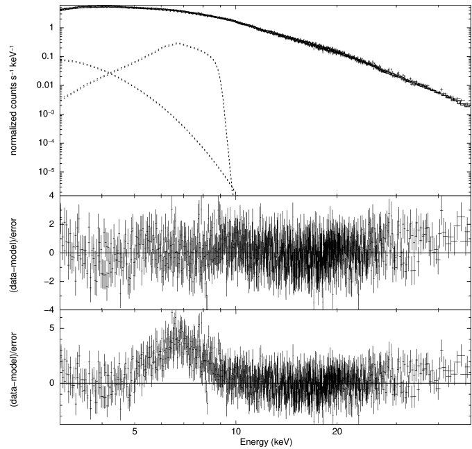
Figure 6. Best-fit NuSTAR spectrum of 4U 1636-53 obtained with the combination of tbabs , kerrconv , diskbb , pexriv and shaddisk , and its residuals in the middle panel; the bottom panel shows the residuals when eliminating the iron line, i.e., accounting for the continuum alone.
