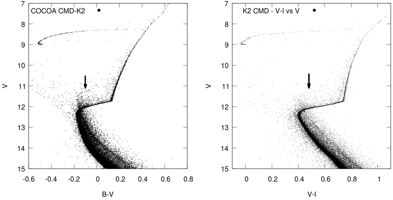
Figure 8. Left Panel: Shows the B-V vs V CMD for the K2 model using instrumental B and V band magnitudes. There are indications of the presence of a second main sequence due to many binaries with q (mass ratio) close to unity. The black arrows shows these binaries that are visible above the MS turn-off. Right Panel: Shows the V-I vs V CMD for the same model which is significantly denser than the K1 model. Due to this higher density and overall lower binary fraction, the photometric errors are larger and it becomes difficult to distinguish the second sequence. Also with higher density, a significant number of such binaries are disrupted. However, there are still binaries with nearly equal mass components above the MS turn-off that are indicated with the black arrow.
