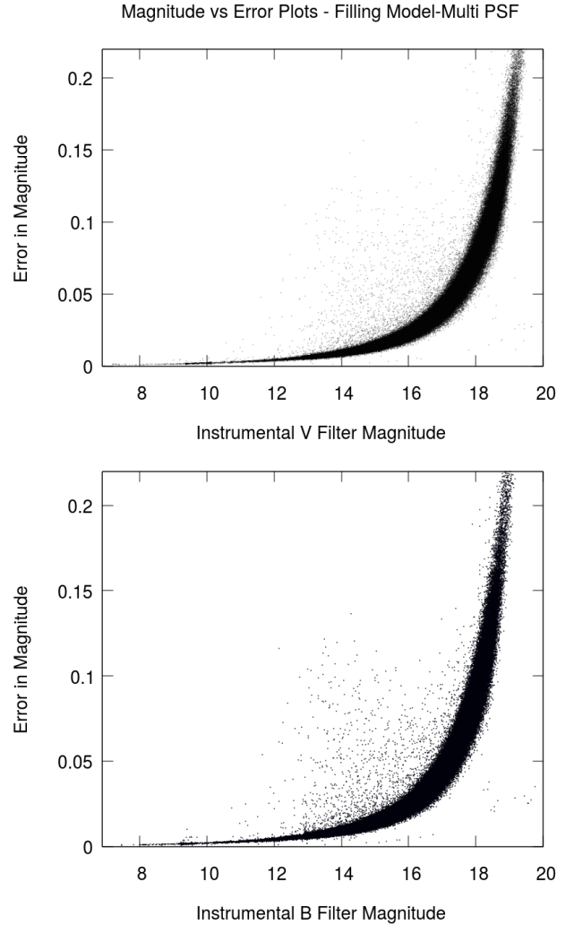
Figure 2. Error vs magnitude plot for V-band and B-band photometry. The x-axis represents the instrumental magnitude and the y-axis represents the error in magnitude.
