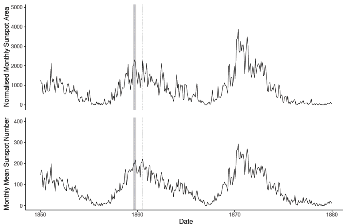
Figure 1: The extreme storms around the Carrington event in 1859 (gray bar) in comparison with the double peak of the monthly mean value of the total sunspot number provided from Sunspot Index and Long-term Solar Observations (SILSO; Clette et al. , 2014; Clette and Lefèvre, 2016) in the lower panel and the monthly mean value of the smoothed sunspot area (Carrasco et al. , 2016) in the upper panel.
